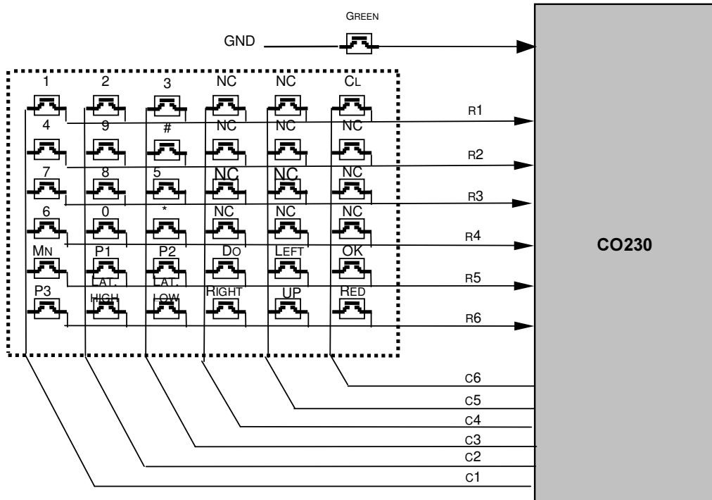
Figure 8 Keyboard connection
