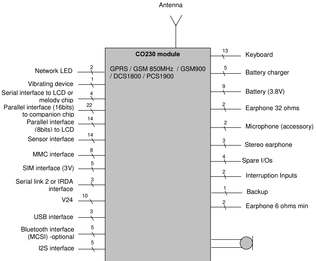
Figure 1 CO230 bloc diagram
