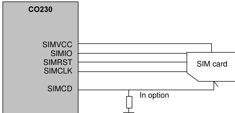
Figure 2 SIM connection
