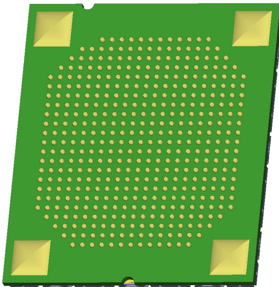
Figure 19 CO230 ballout side
