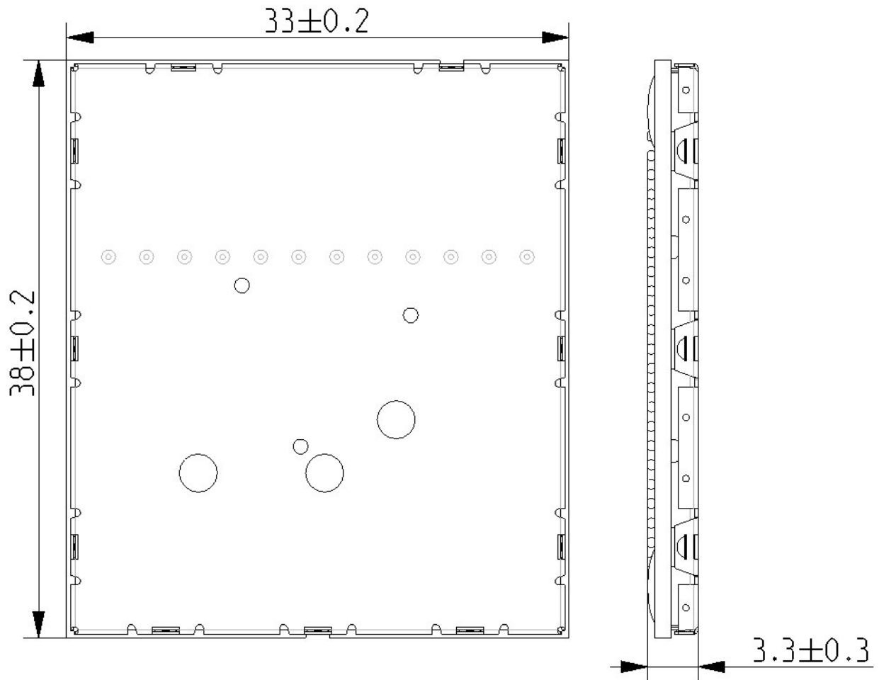
Figure 20 CO230 dimensions
