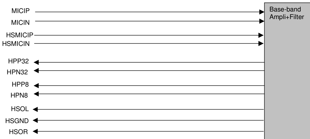
Figure 3 Audio
