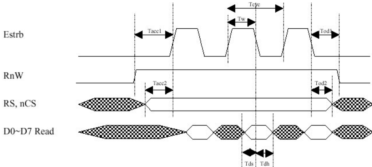
Figure 6 Read timing (in 6800 mode)
