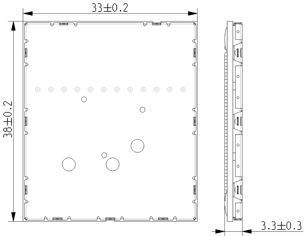
Figure 20 CO2xx/XS200 dimensions
