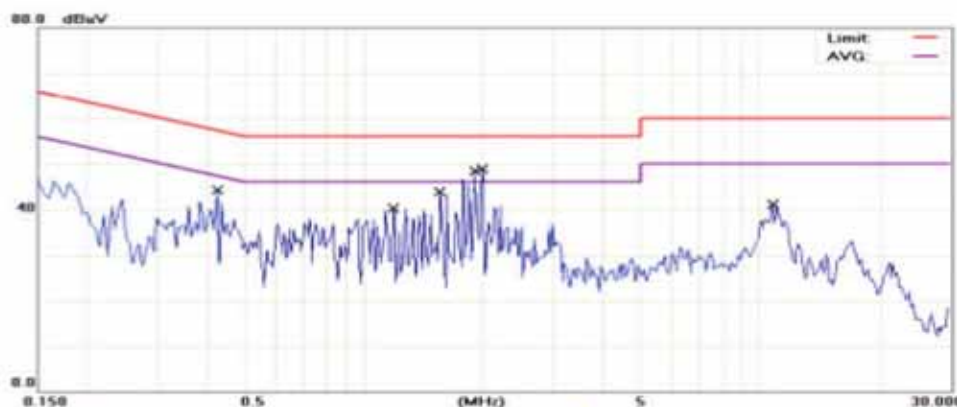
Conducted Emission Measurement
