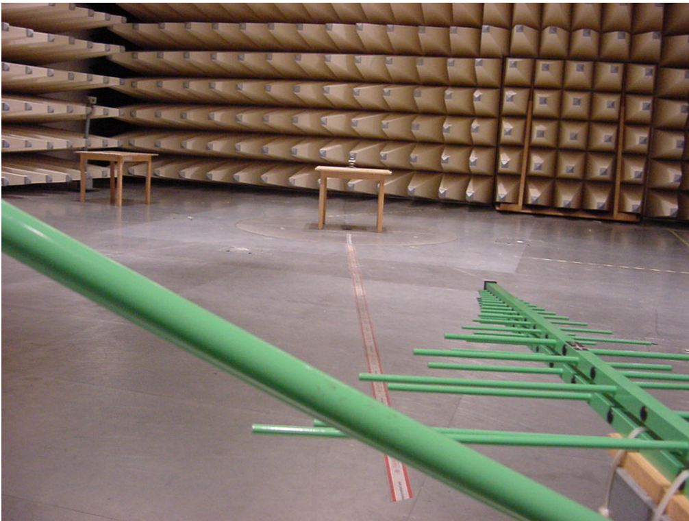
Photo 4 (Radiated Emissions):
