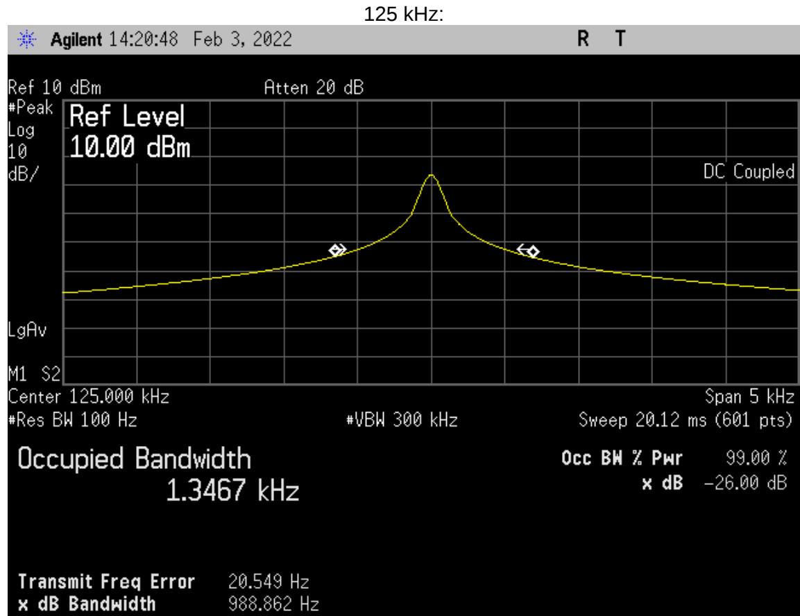
Figure 5. Occupied Bandwidth Plots
