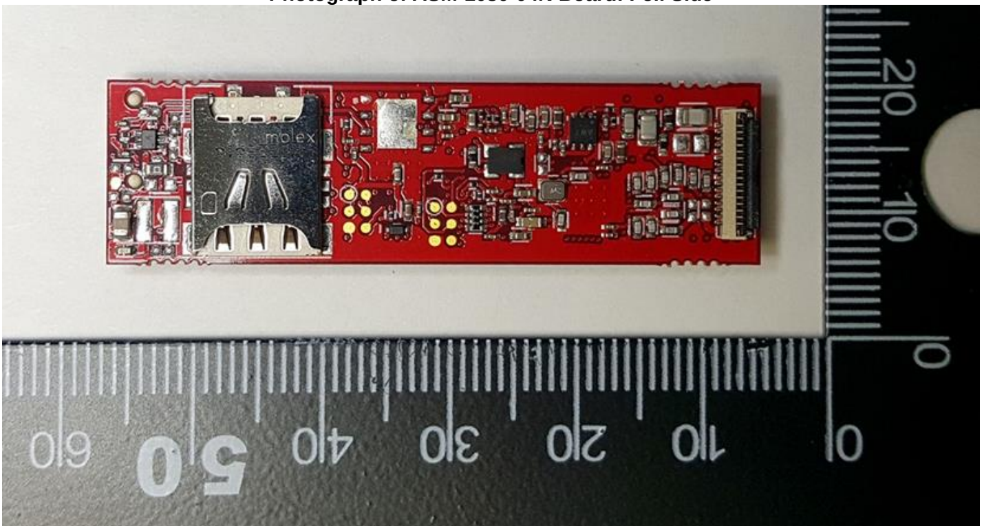
Photograph of ASM-1080-04N Board: Foil Side
