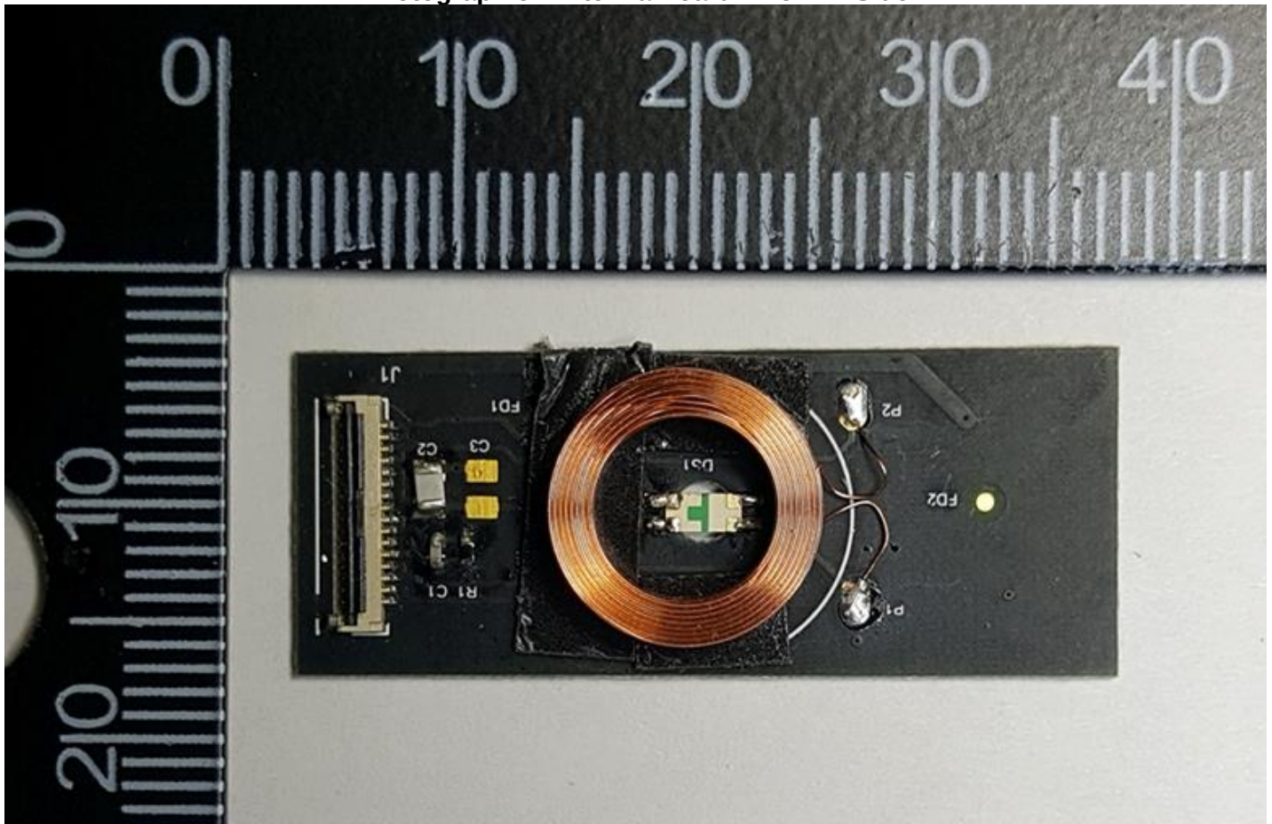
Photograph of Antenna Board: 125 kHz Side
