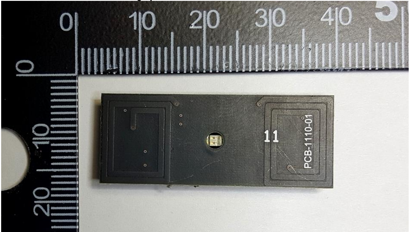
Photograph of Antenna Board: 125 kHz Side
