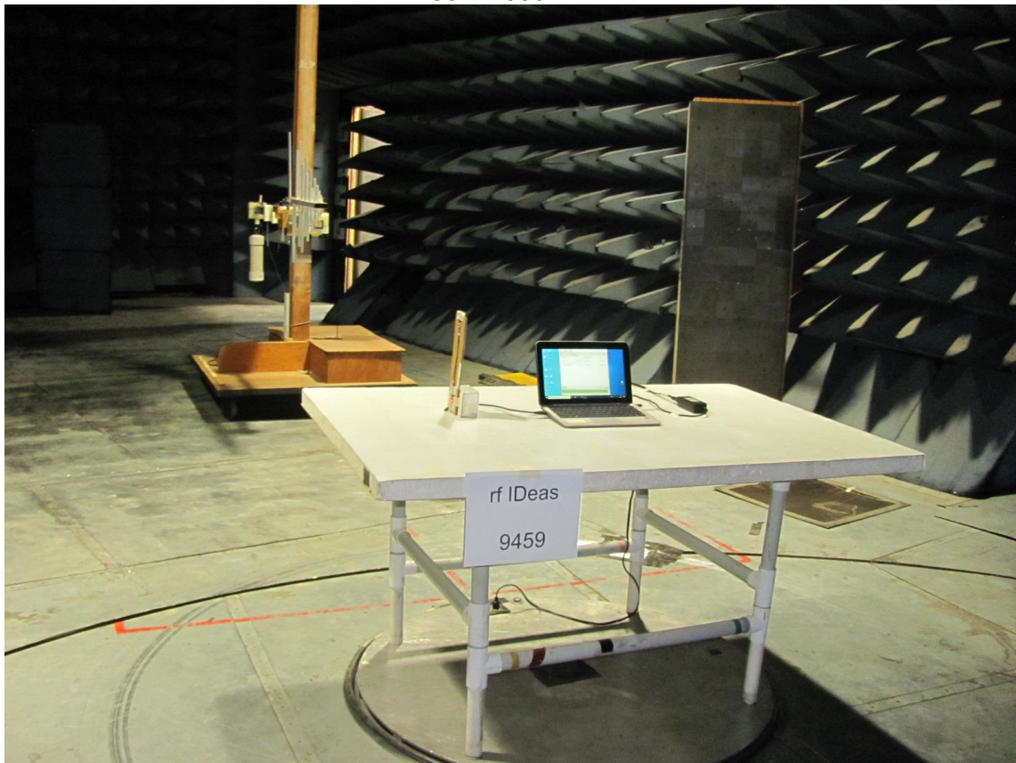
250 – 1000 MHz
