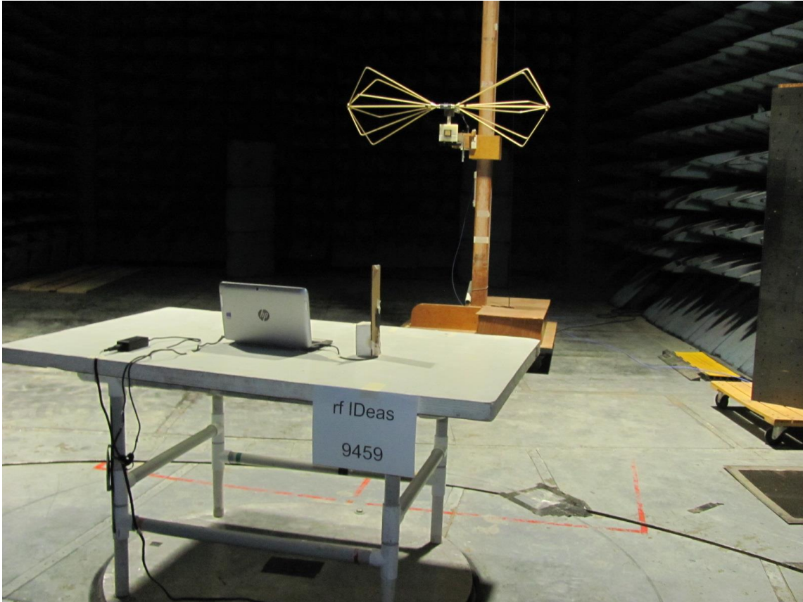
30 – 250 MHz
