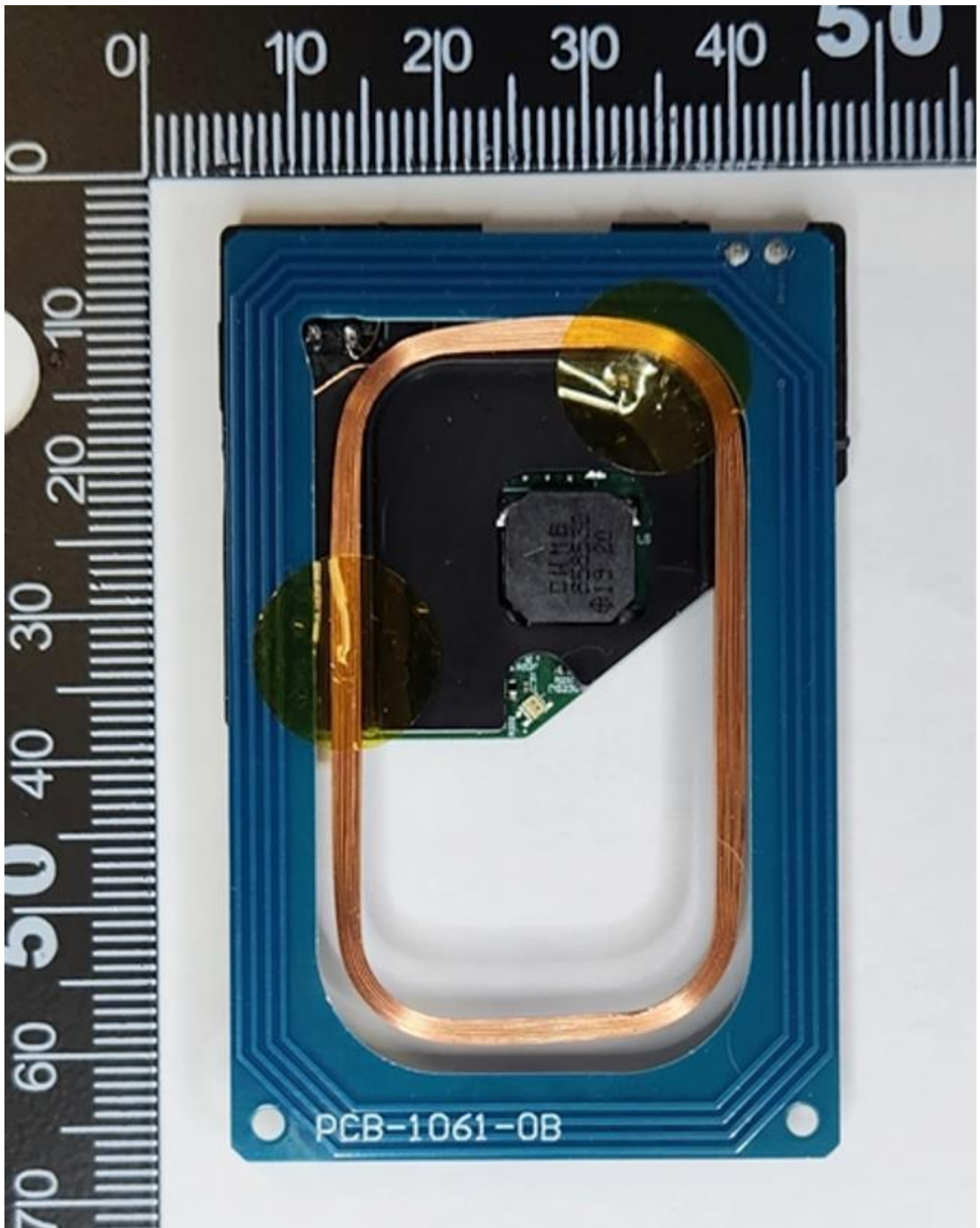
Photographs of Antenna: Top
