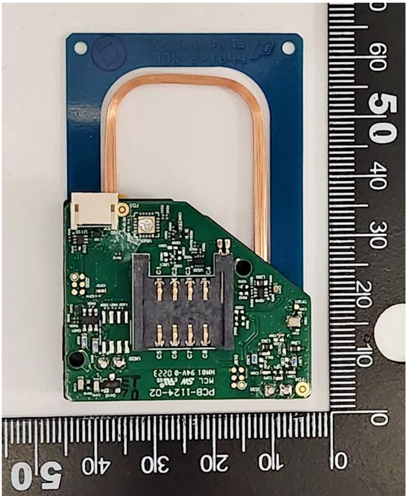
PCB's for SP80200: Front
