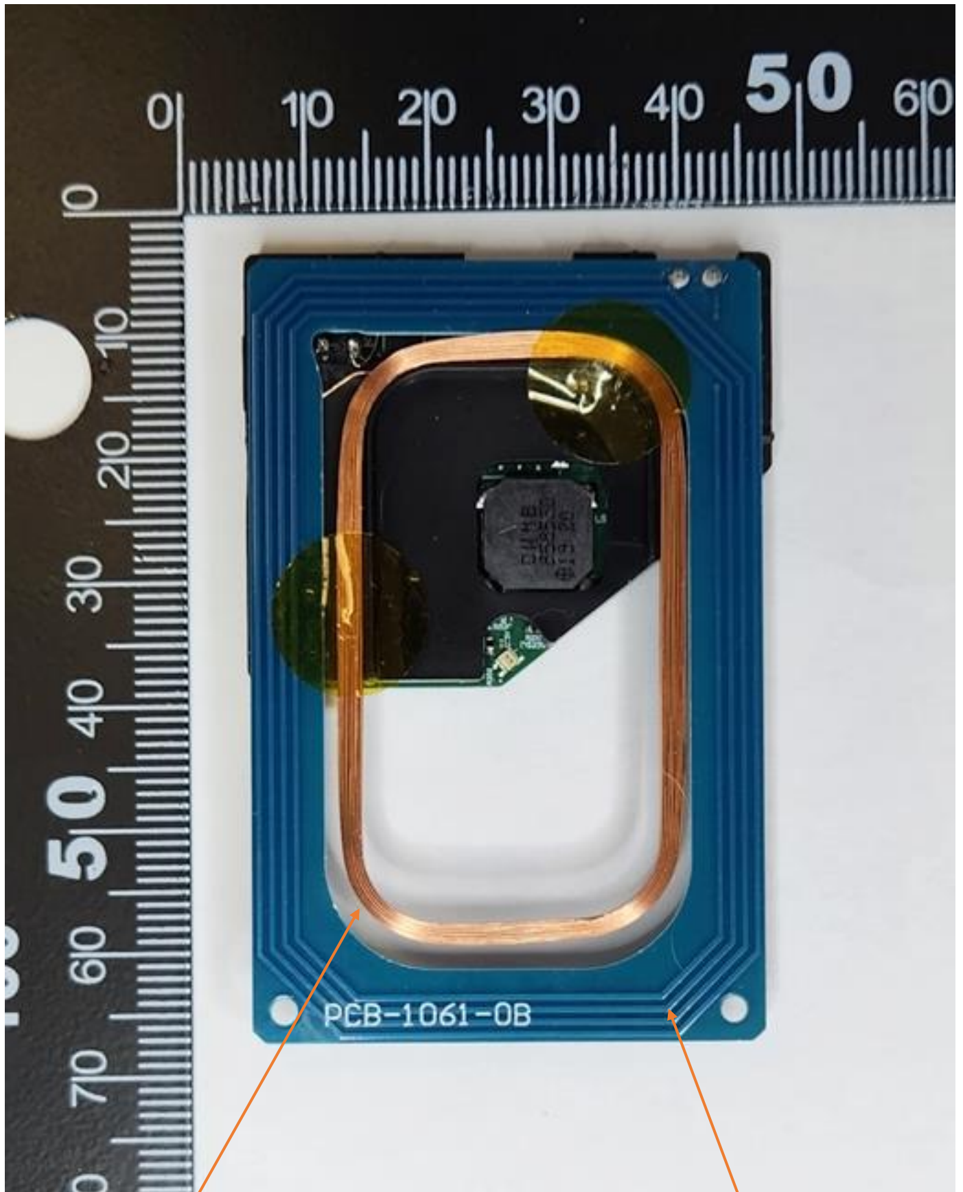
125 kHz Antenna
