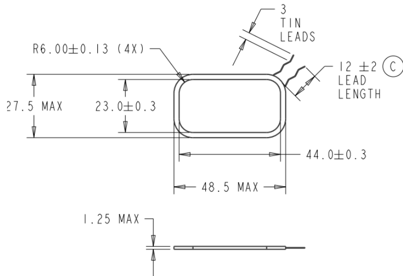
125 kHz Antenna Details.
