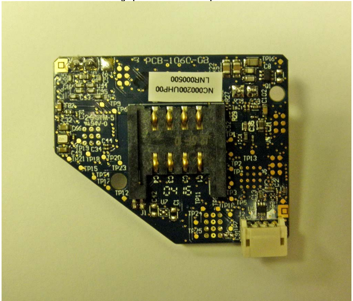
Photograph of PC Board: Component Side
