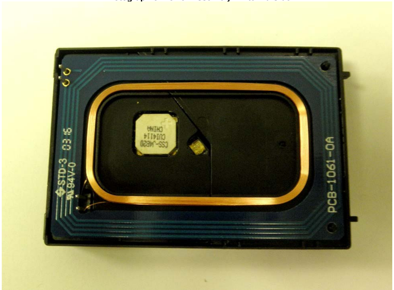
Photograph of Lower Assembly: Antenna Side
