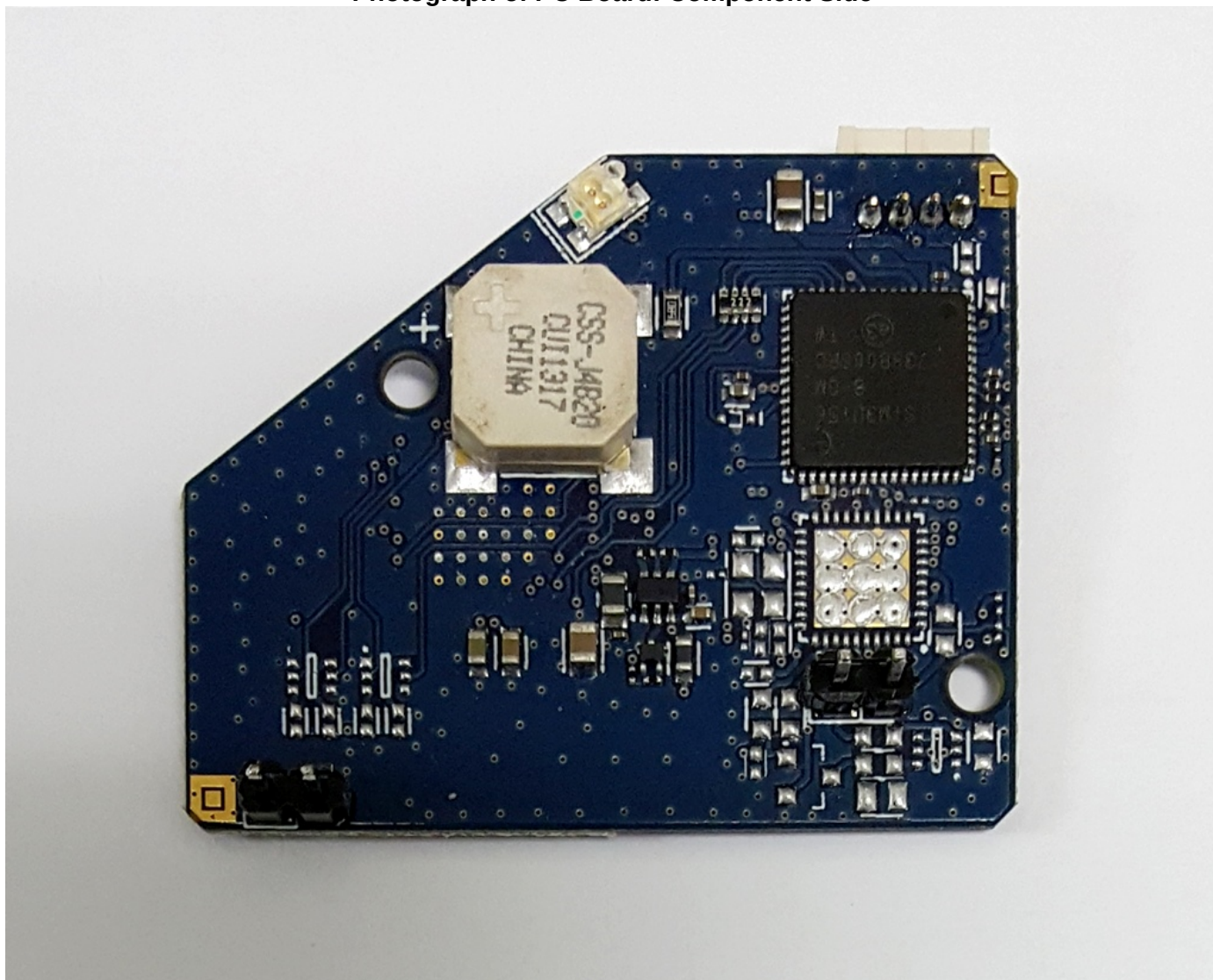
Photograph of PC Board: Component Side
