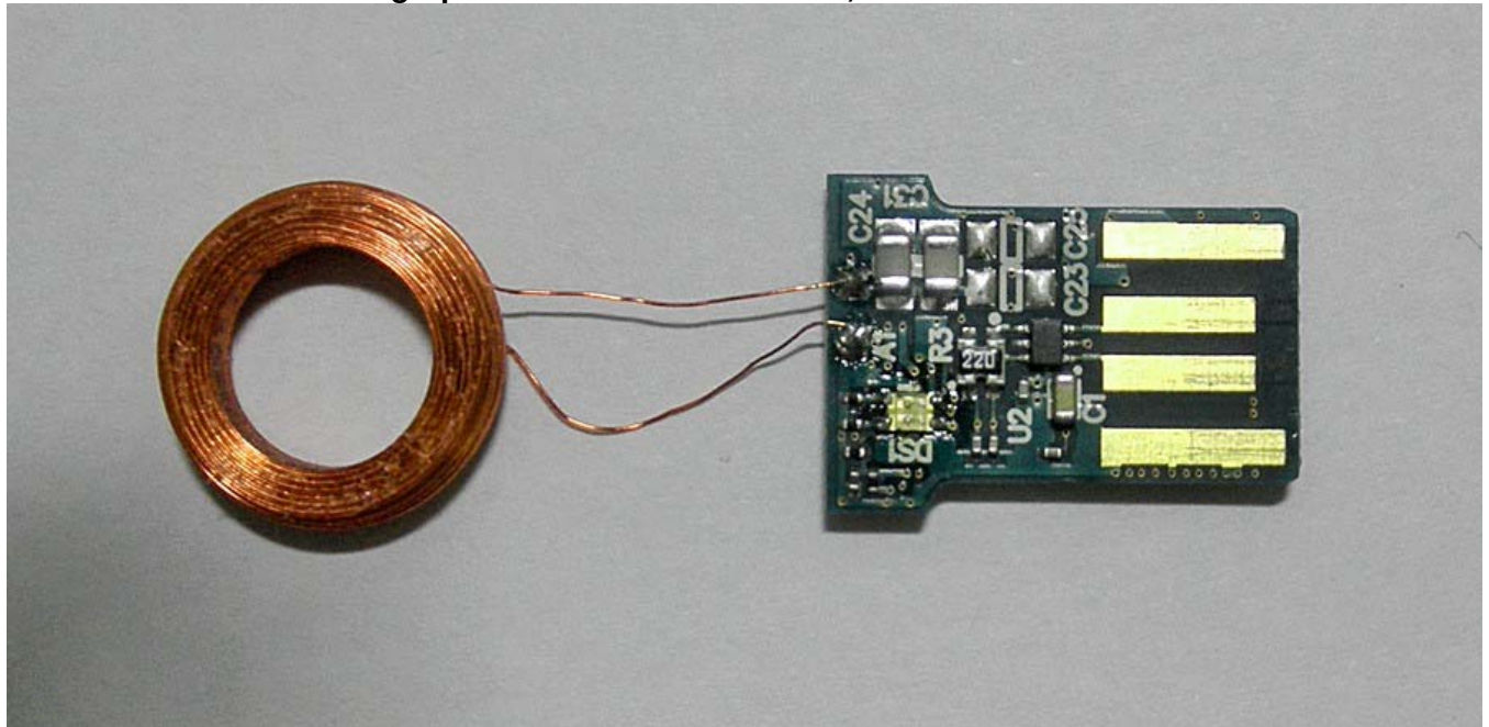
Photograph of PC Board: Component Side
