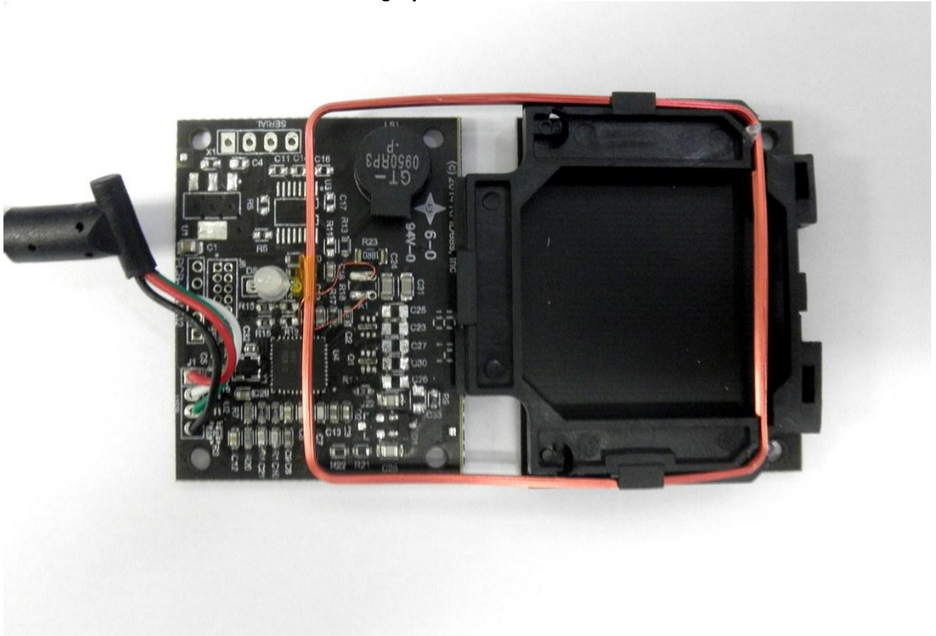
Photograph of Antenna
