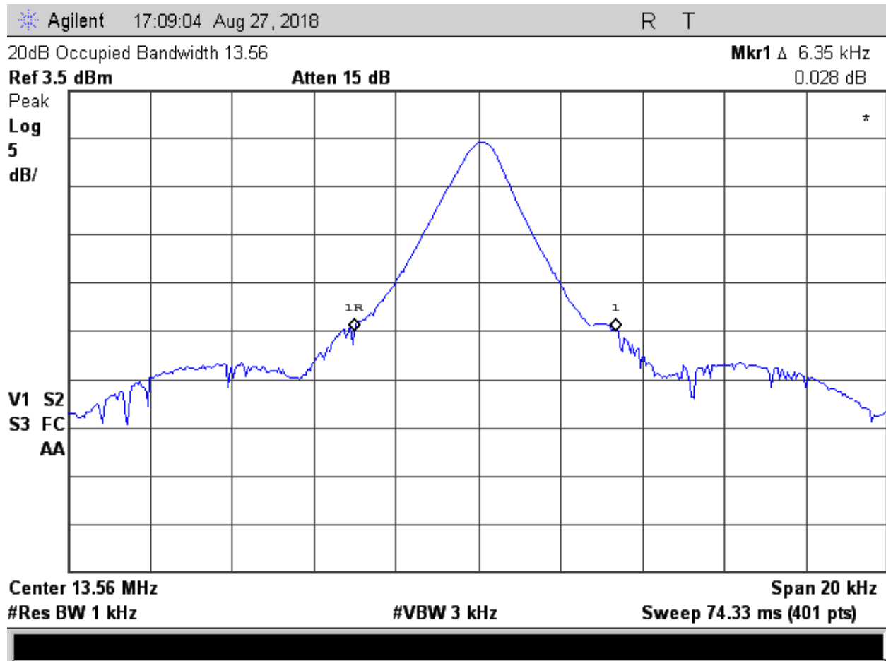
Figure 3. Occupied Bandwidth Plots 13.56 MHz
