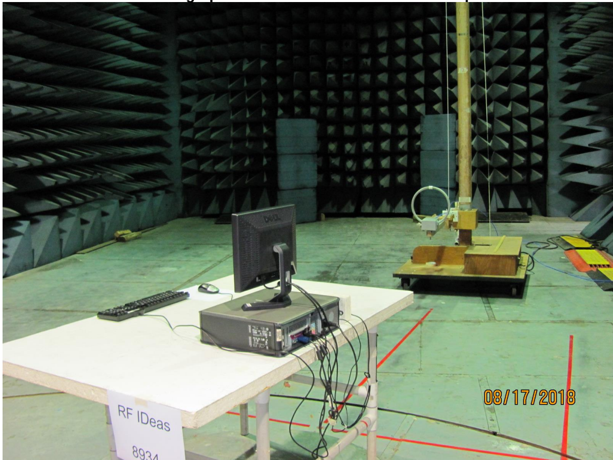
Photograph of Radiated Emissions Test Setup
