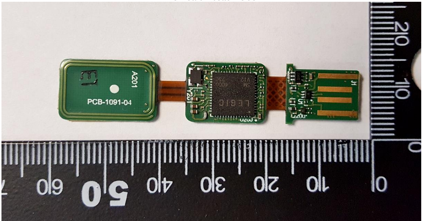
PC Board - bottom side
