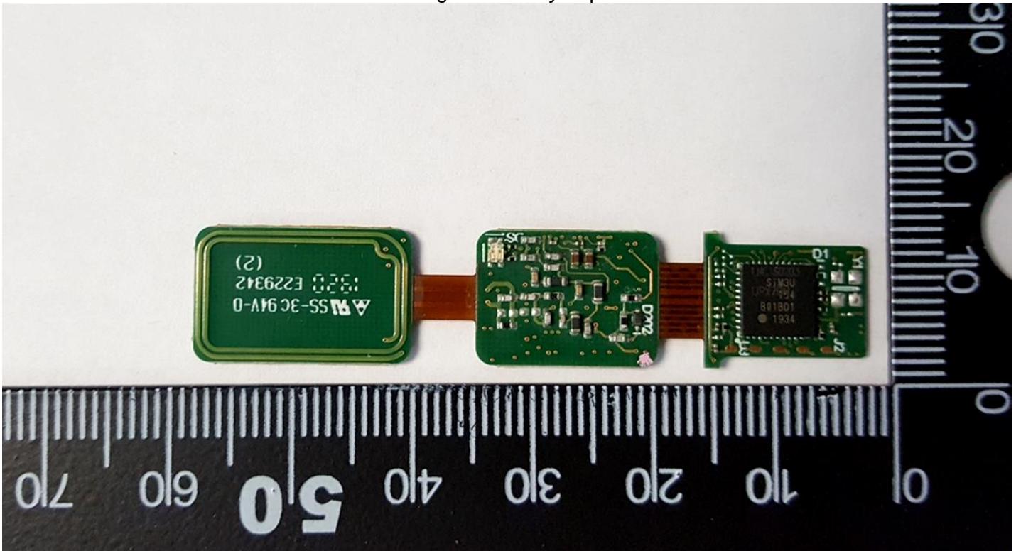
Legic Assembly Top
