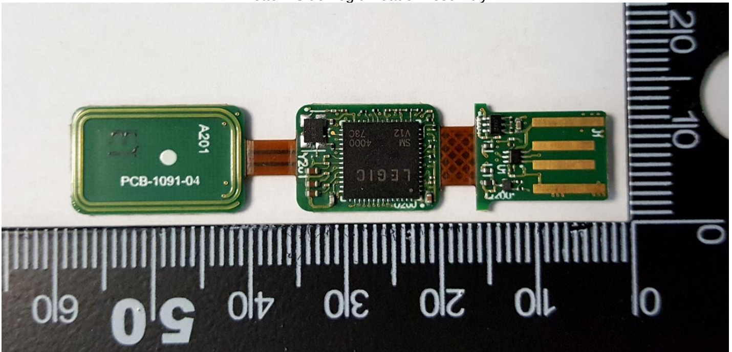
Bottom Side Legic Reader Assembly
