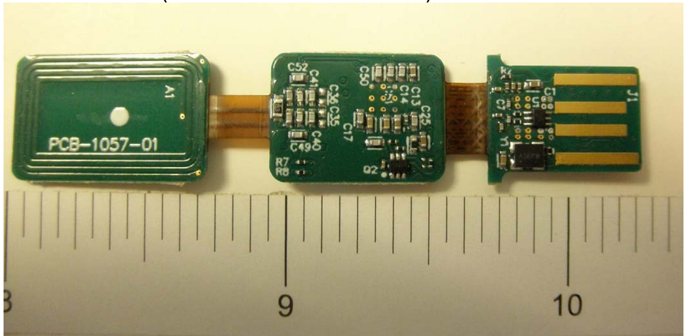
Photograph of PC Board: Foil Side Both models (RDR-7011XAKU and RDR-7511XAKU) look the same in this view
