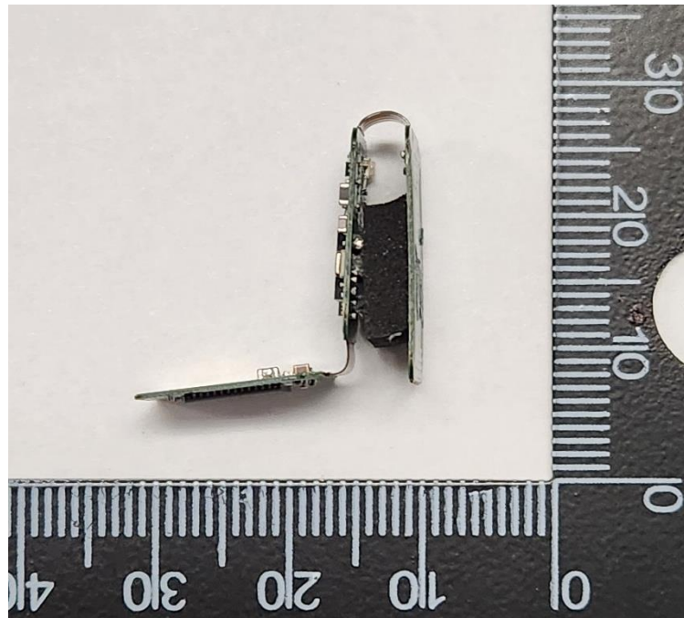
Side view of circuit boards assembled
