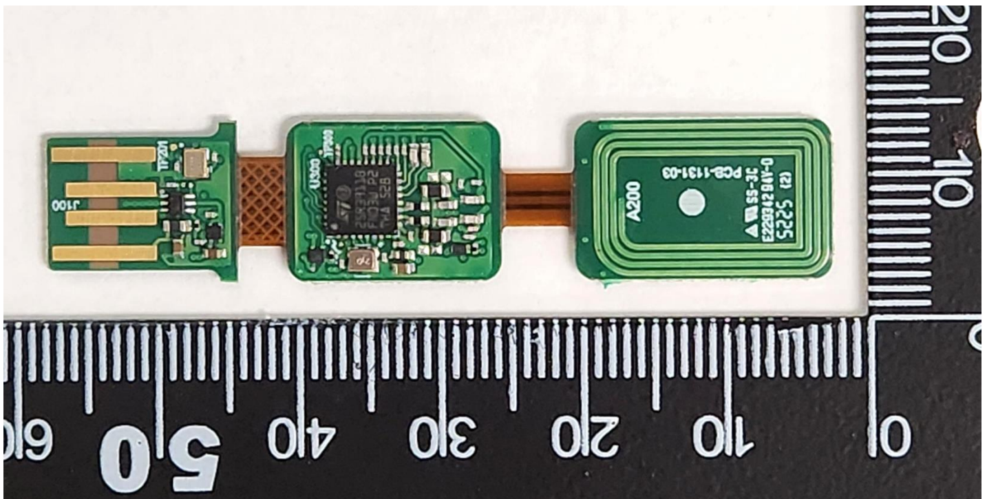
Both sides of all circuit boards
