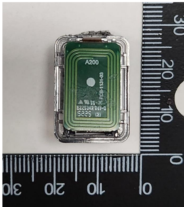
Housing open
