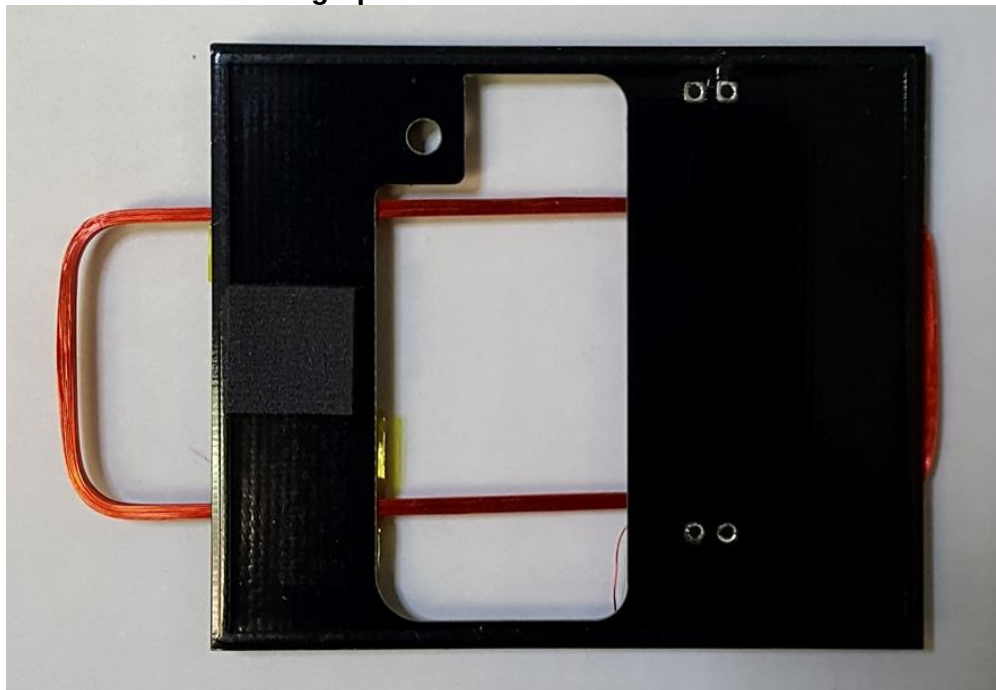
Photograph of Antenna Board: Foil side
