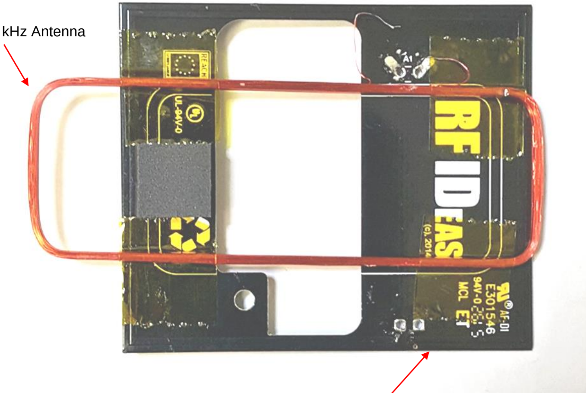
Photograph of Antenna Board: Component side
