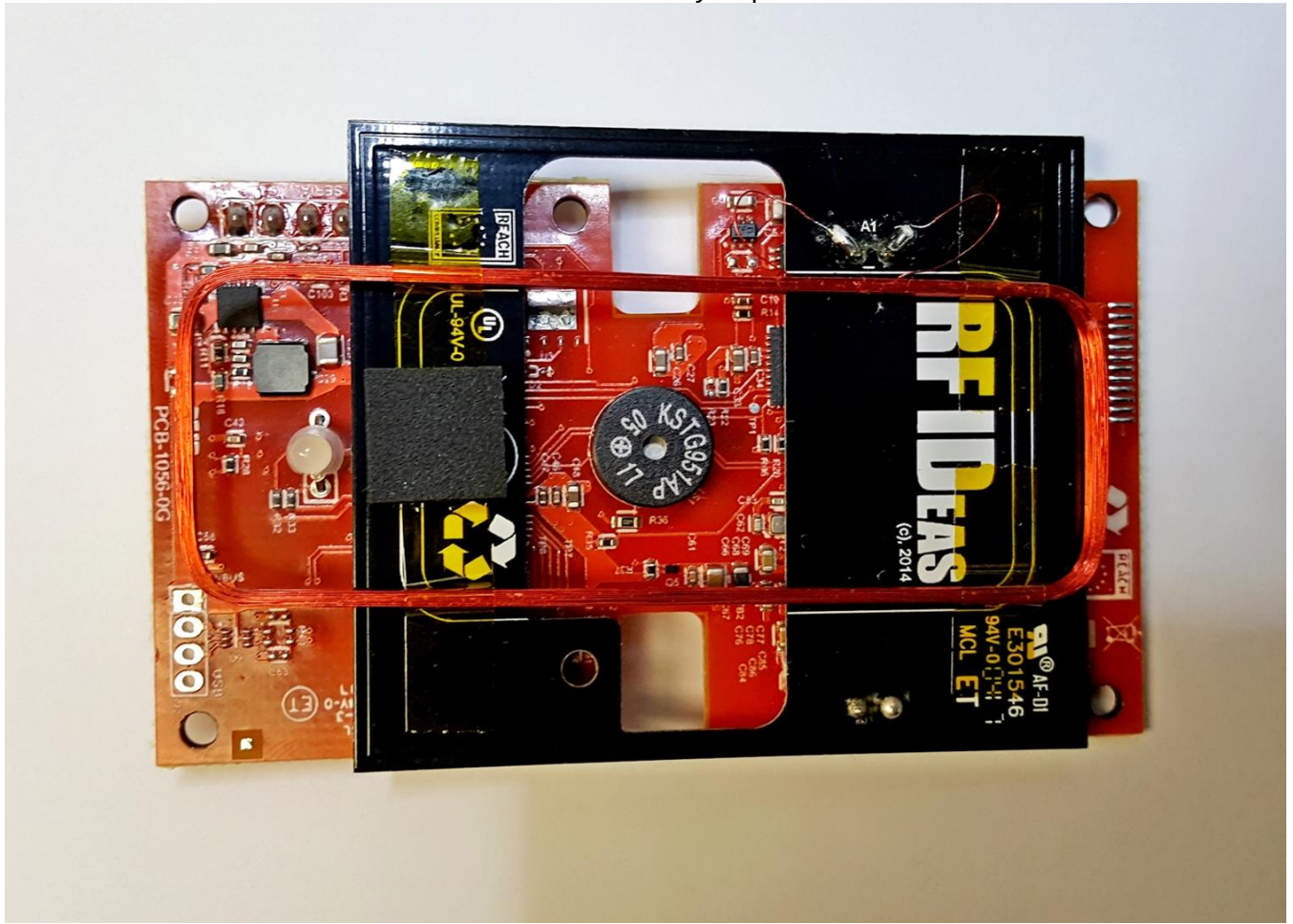
EUT Assembly-Top Cover removed
