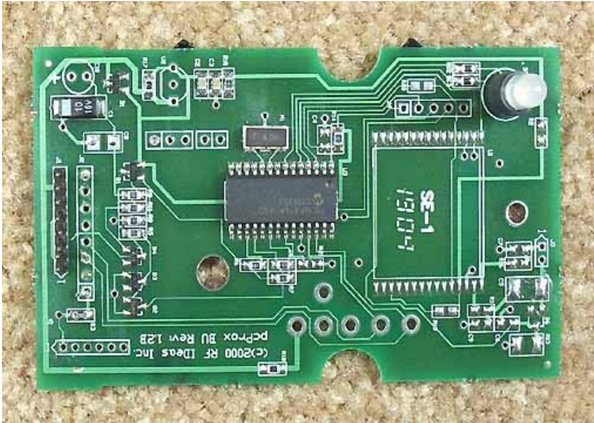
Antenna PCB Top 232
