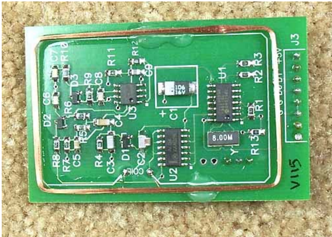
Antenna PCB Top USB
