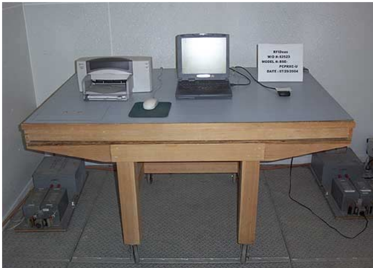
Conducted Emissions - Front View - USB
