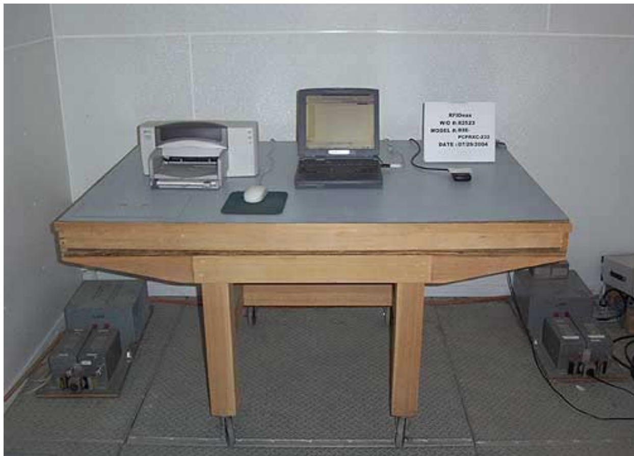
Conducted Emissions - Front View - 232
