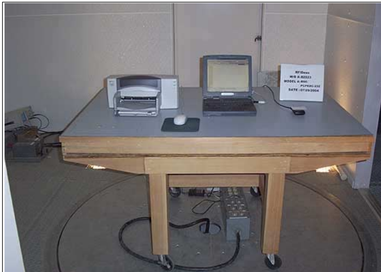
Radiated Emissions - Front View - 232
