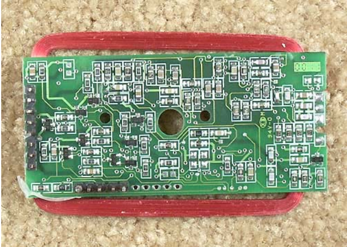
Antenna PCB Bottom USB
