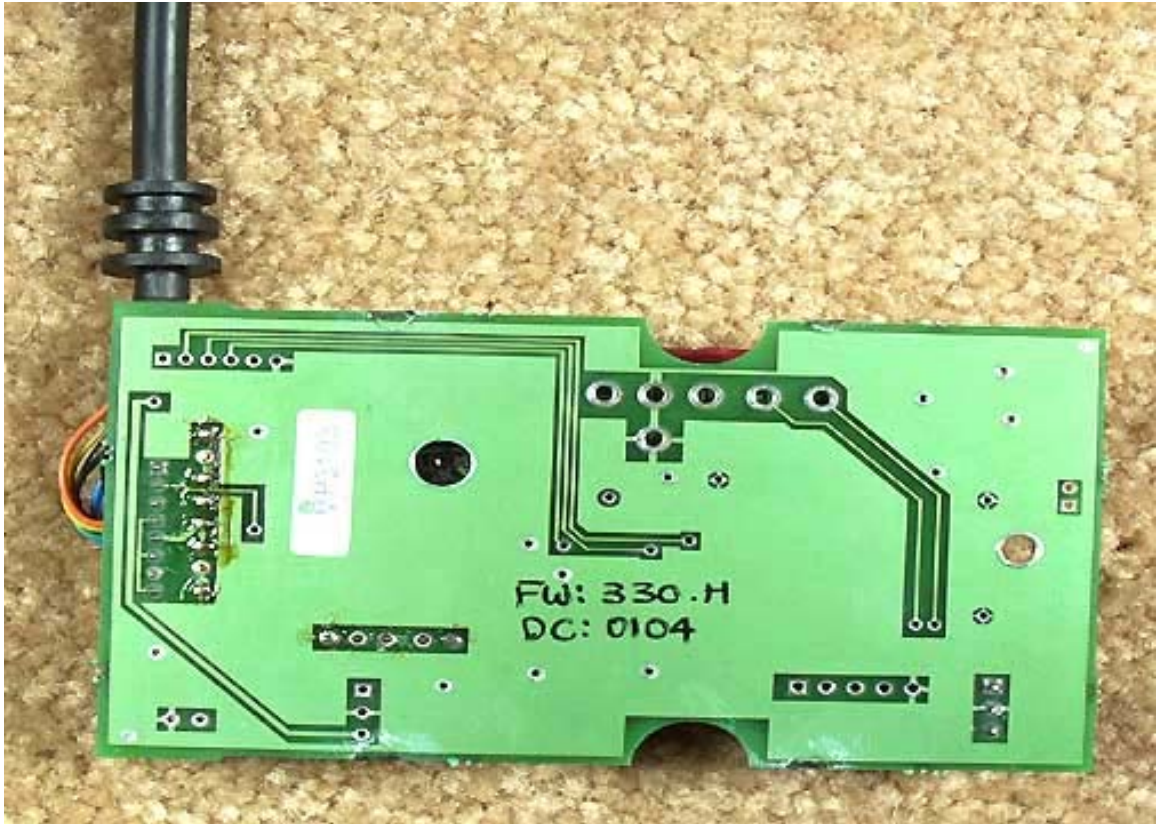
Main PCB Back 232
