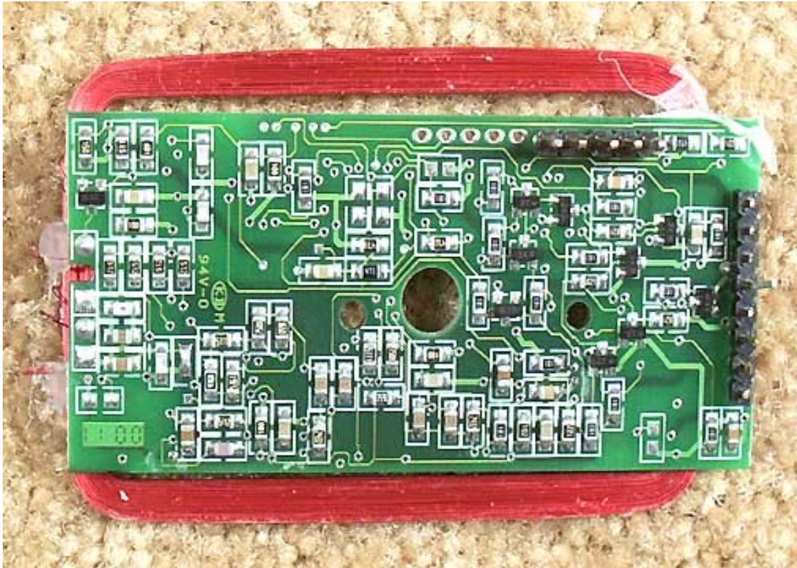
Antenna PCB Back 232
