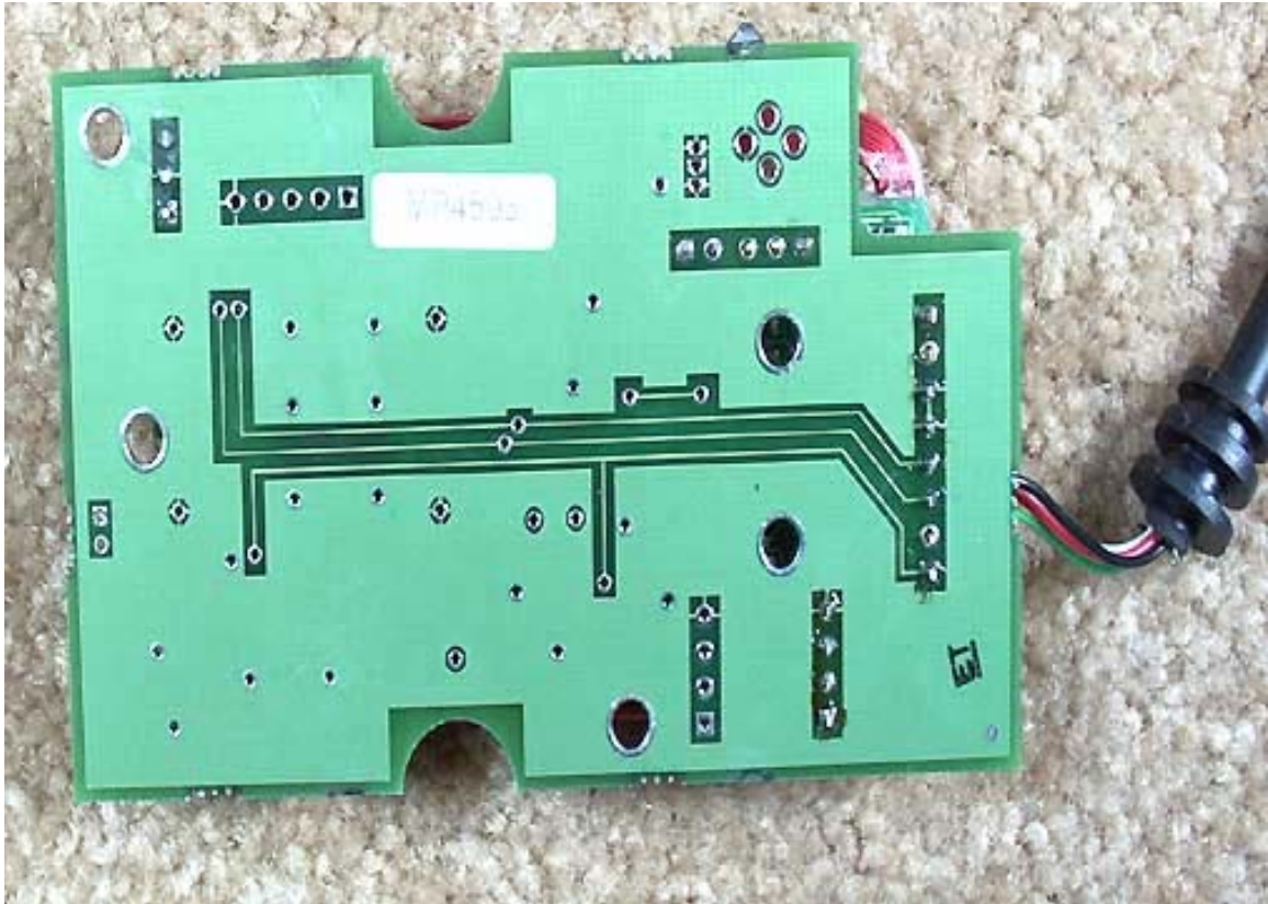
Main PCB Bottom USB
