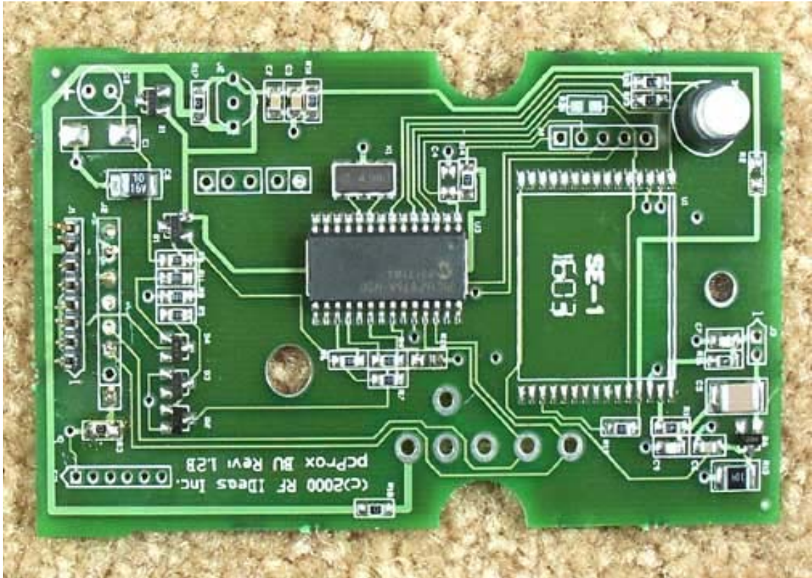
Main PCB Top 232
