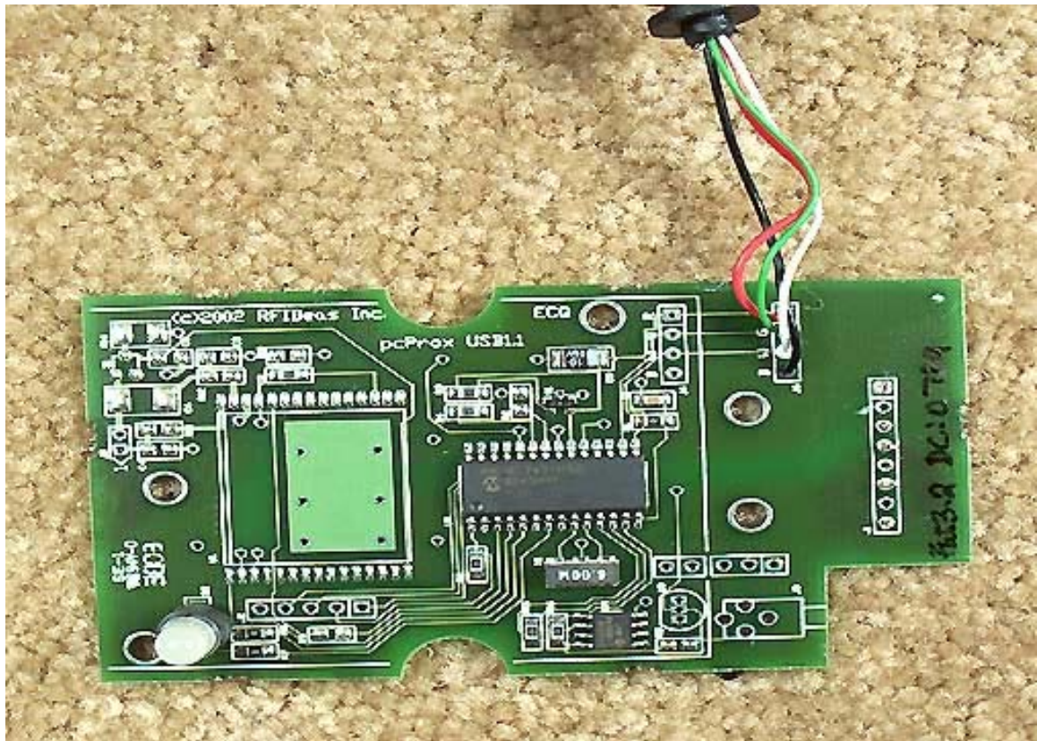
Main PCB Top USB
