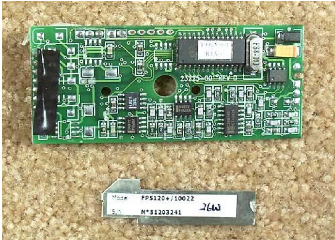
Antenna PCB Top No Shield
