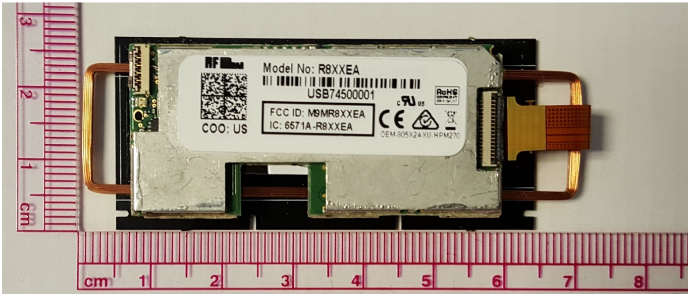
Assembly: Top view
