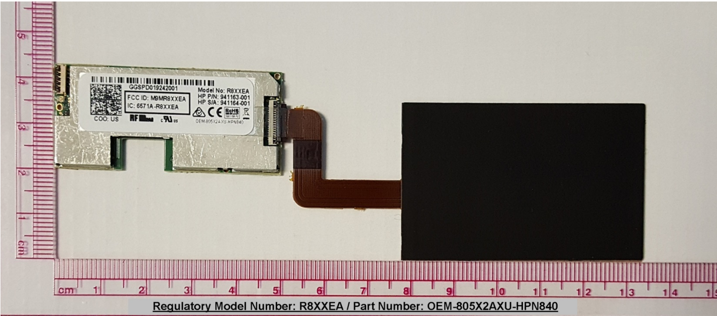
Assembly: Top view
