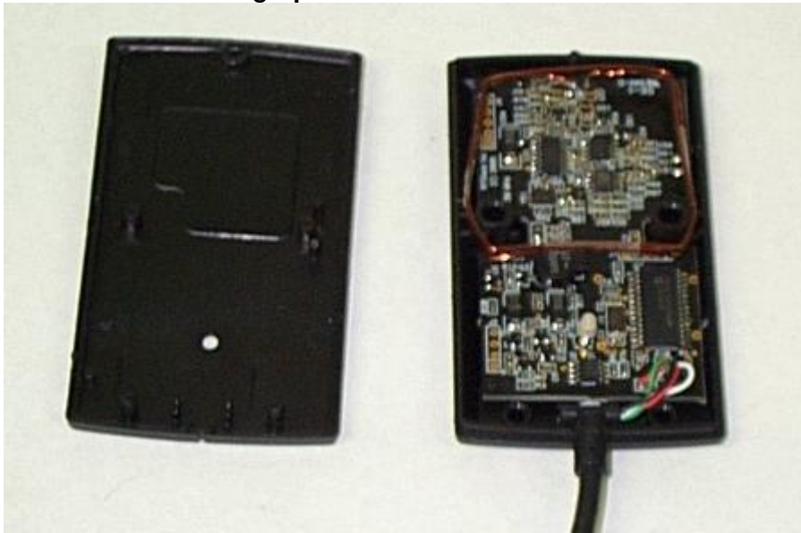
Photograph of PCB: Front
