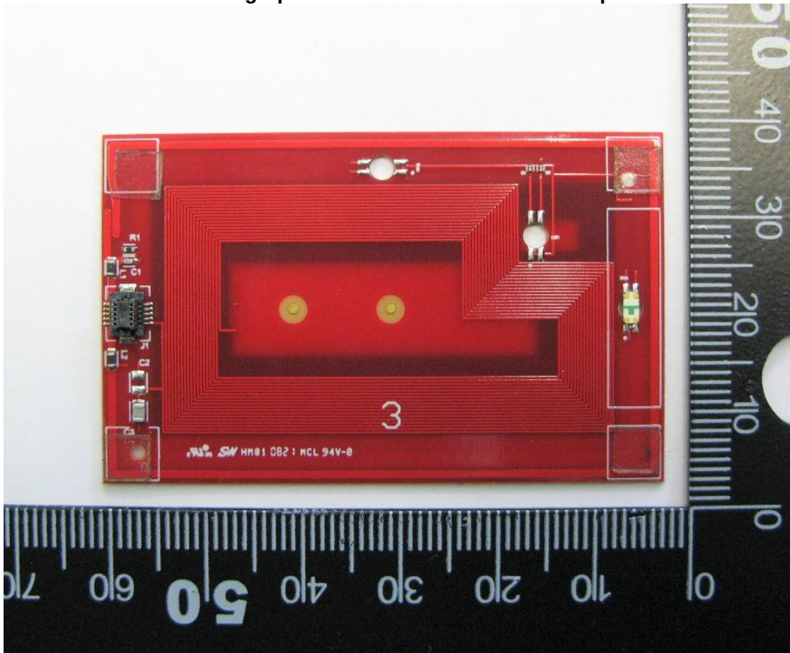
Photograph of 1098-07 Antenna Board: Bottom
