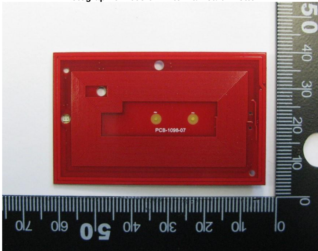
Photograph of 1098-07 Antenna Board: Bottom
