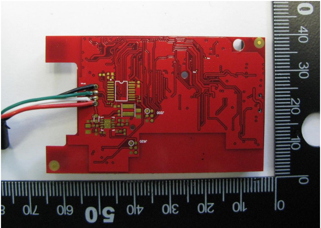
PCB: Foil Side
