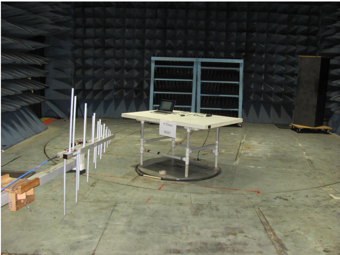
250 – 1000 MHz
