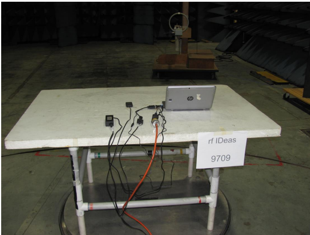
External Power supply
