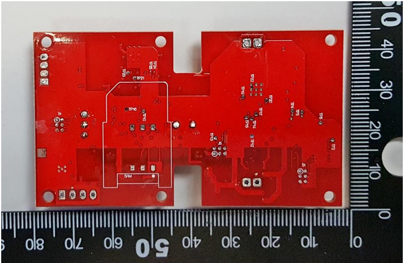
PCB: Foil Side
