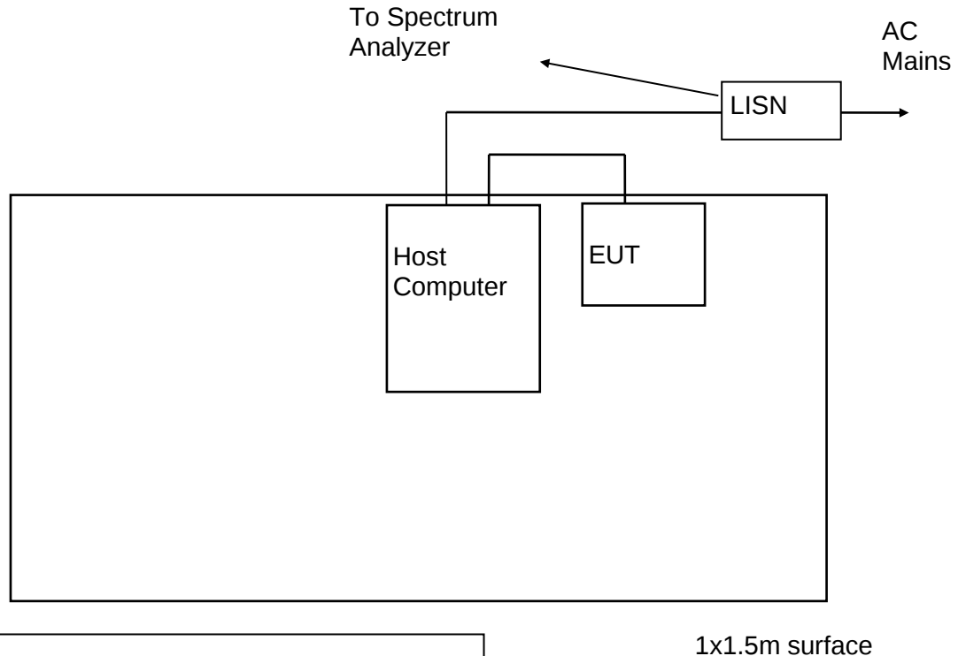
Figure 1. Conducted Emissions Test Setup
