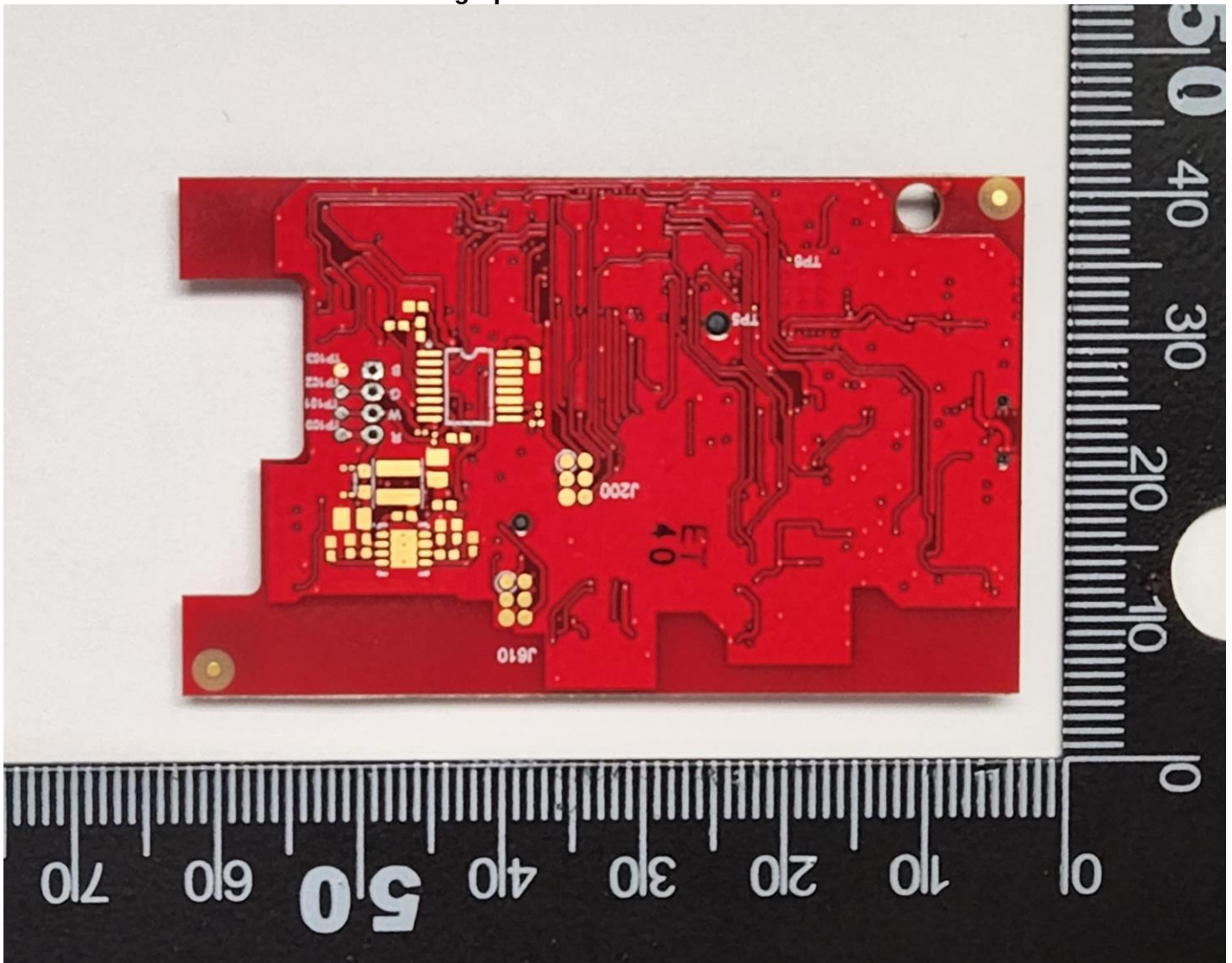
Photograph of 305 PC Board: Foil Side
