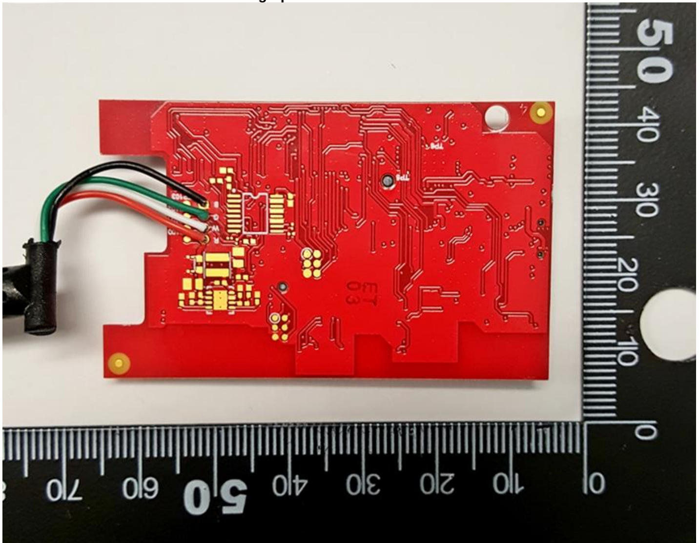
Photograph of 300 PC Board: Foil Side
