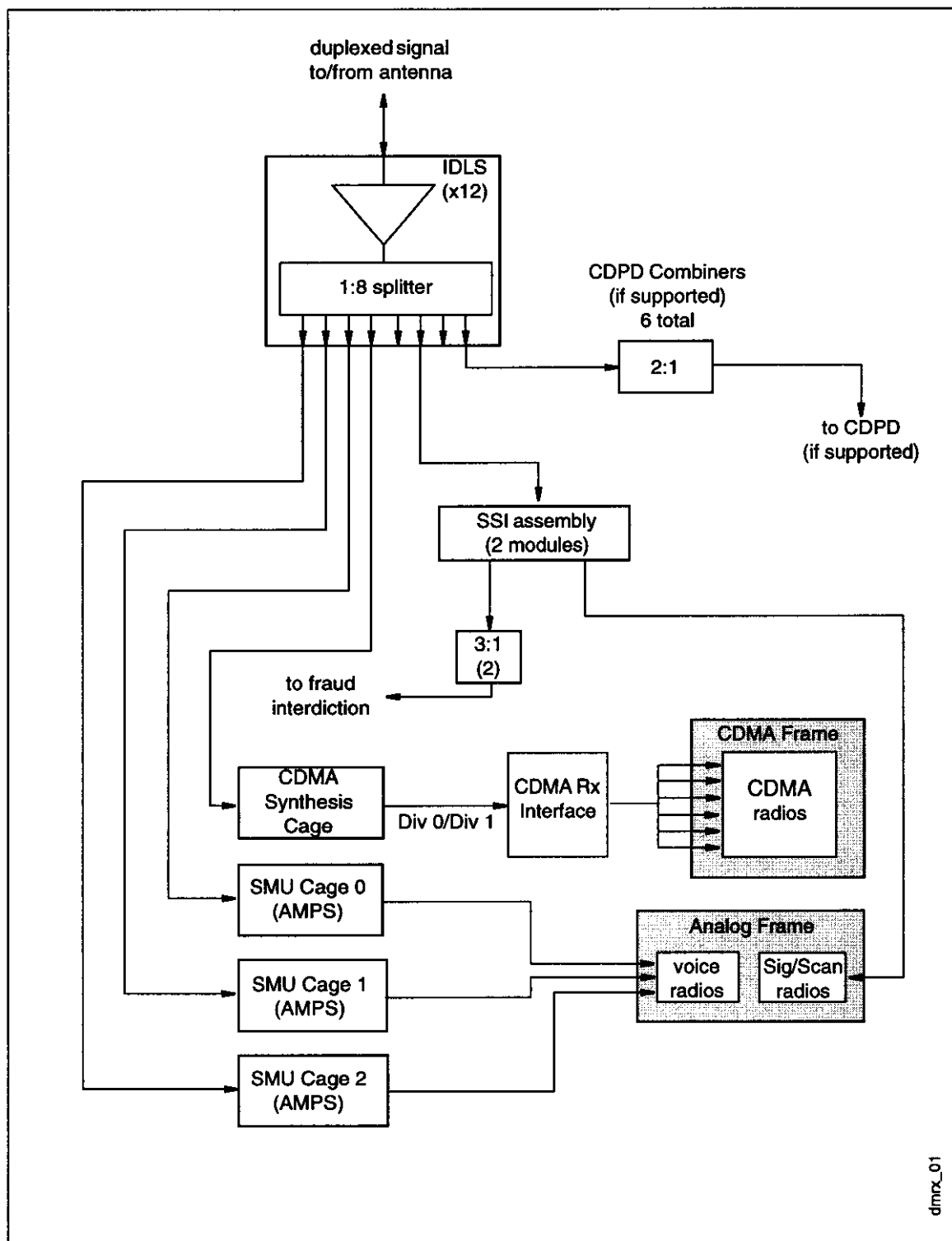
Figure 1.1 SpotLight 2000 Dual-Mode Receive RF Path
