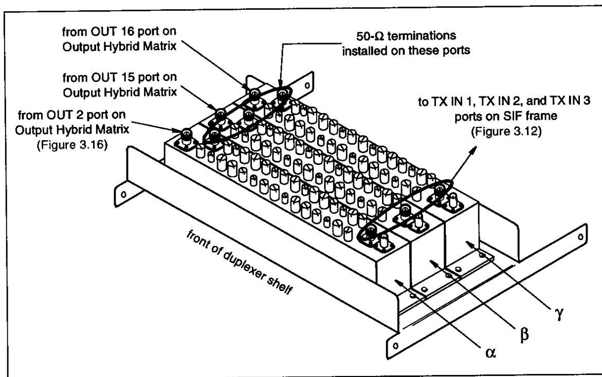
Figure 3.11 Duplexer Shelf
