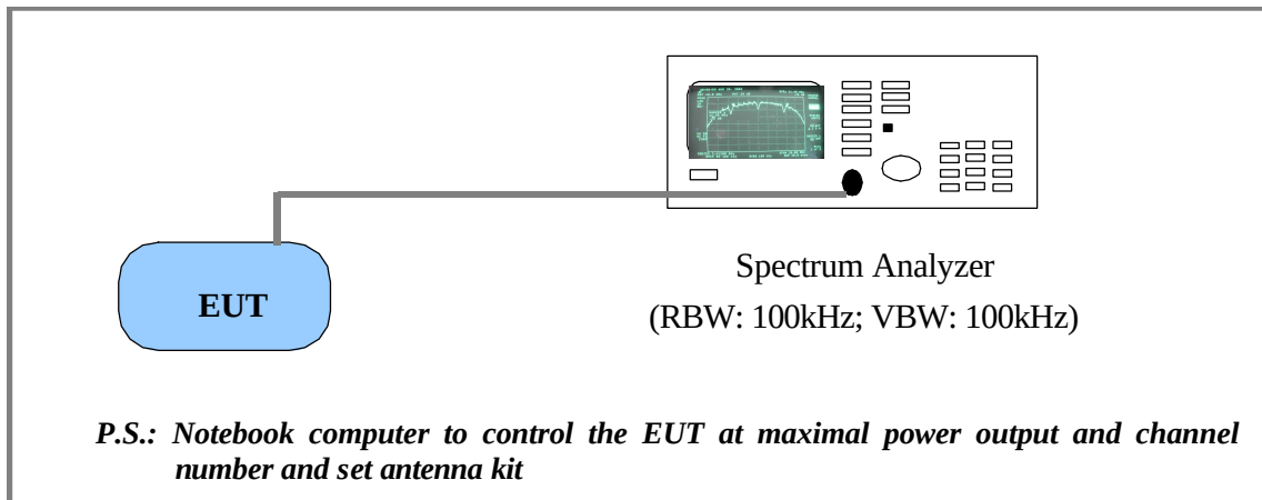
Test Configuration of Bandwidth for Direct Sequence System
