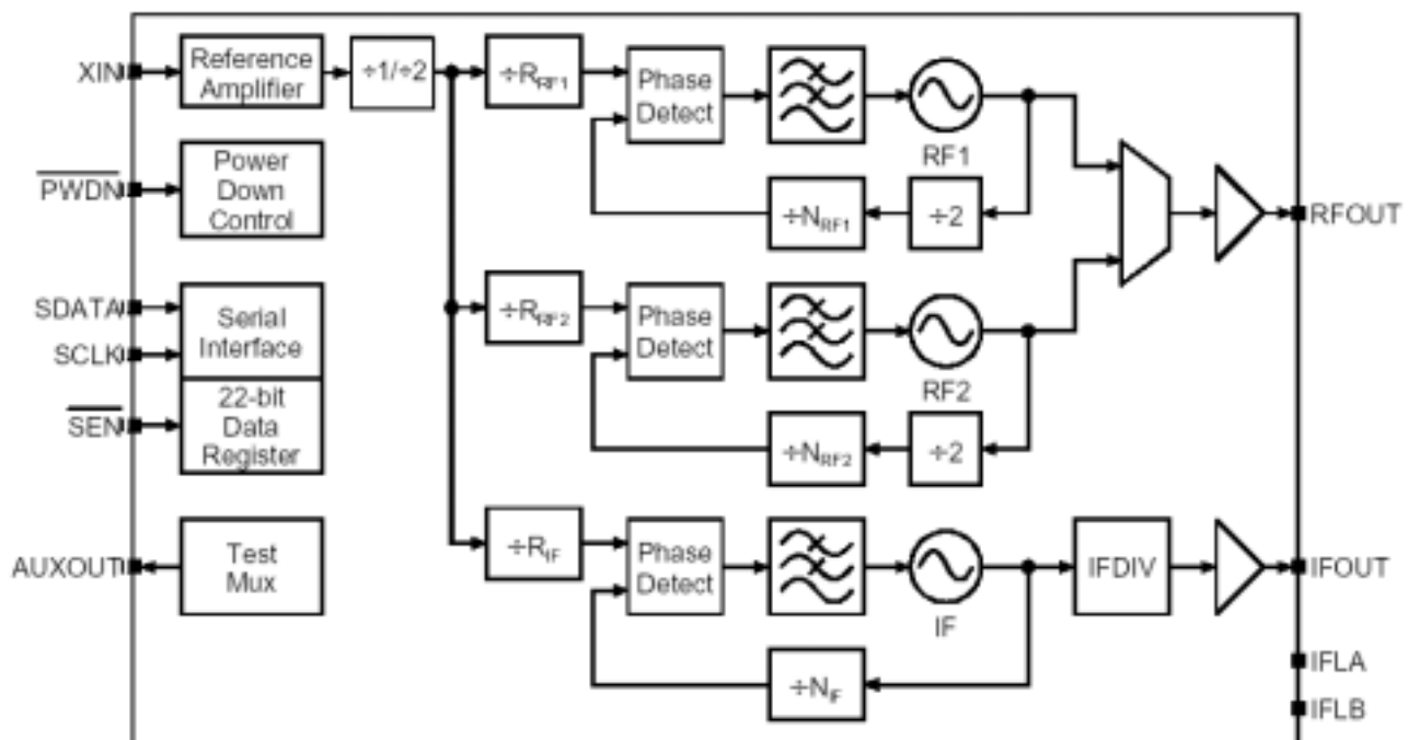
Figure 10. Si4126 Block Diagram
