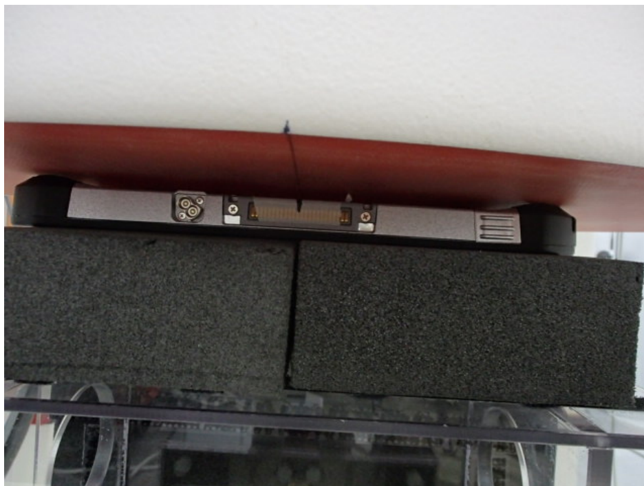
Main and Auxiliary Antenna, Rear, 0mm Separation Distance
