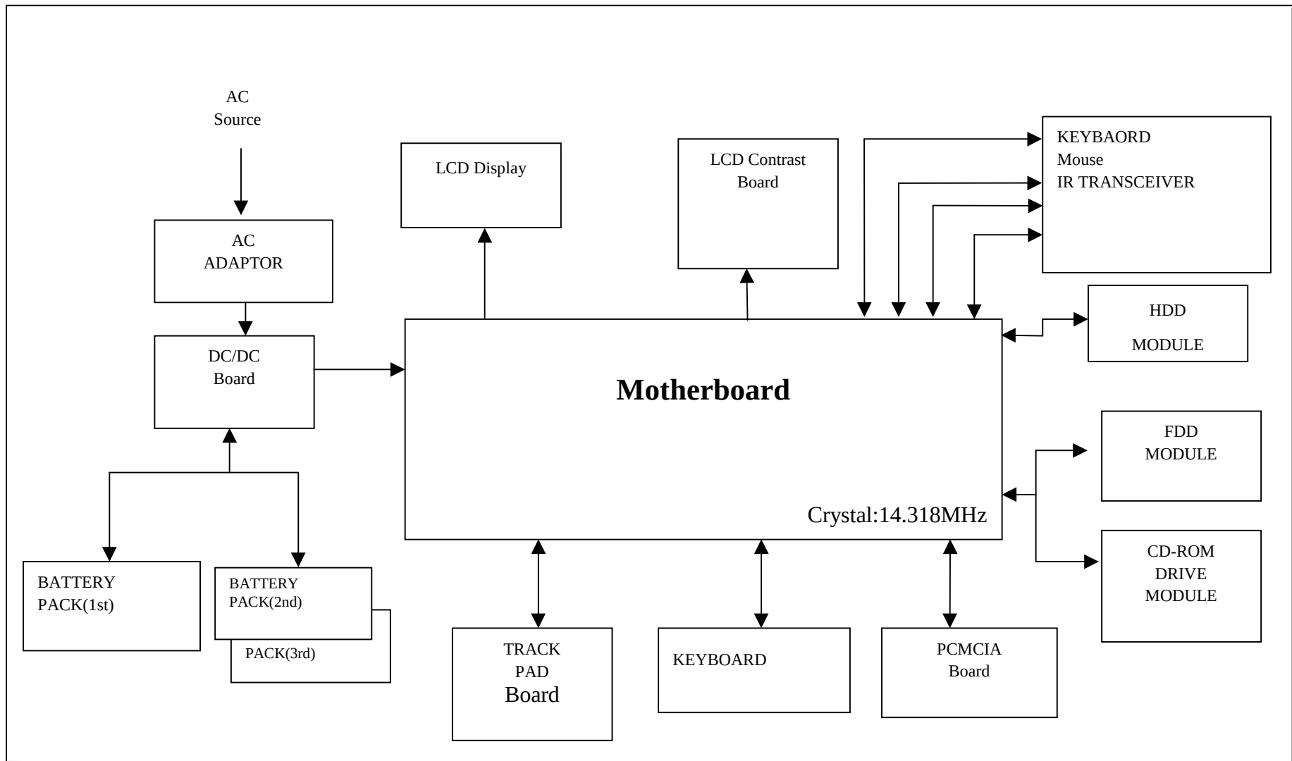
Figure - System Block Diagram
