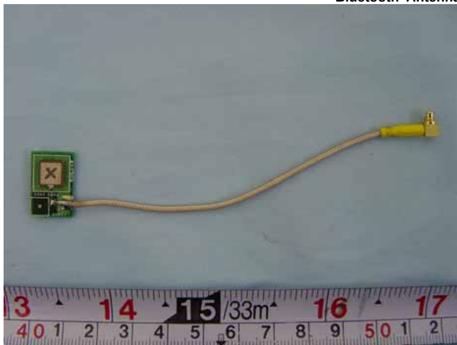
Bluetooth Antenna
