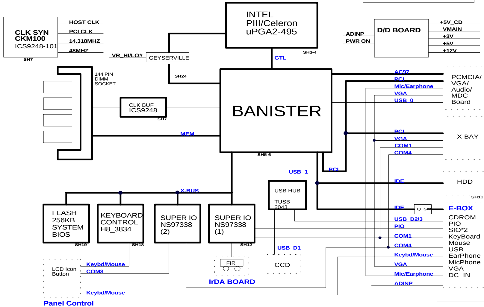
CA25 Block Diagram
