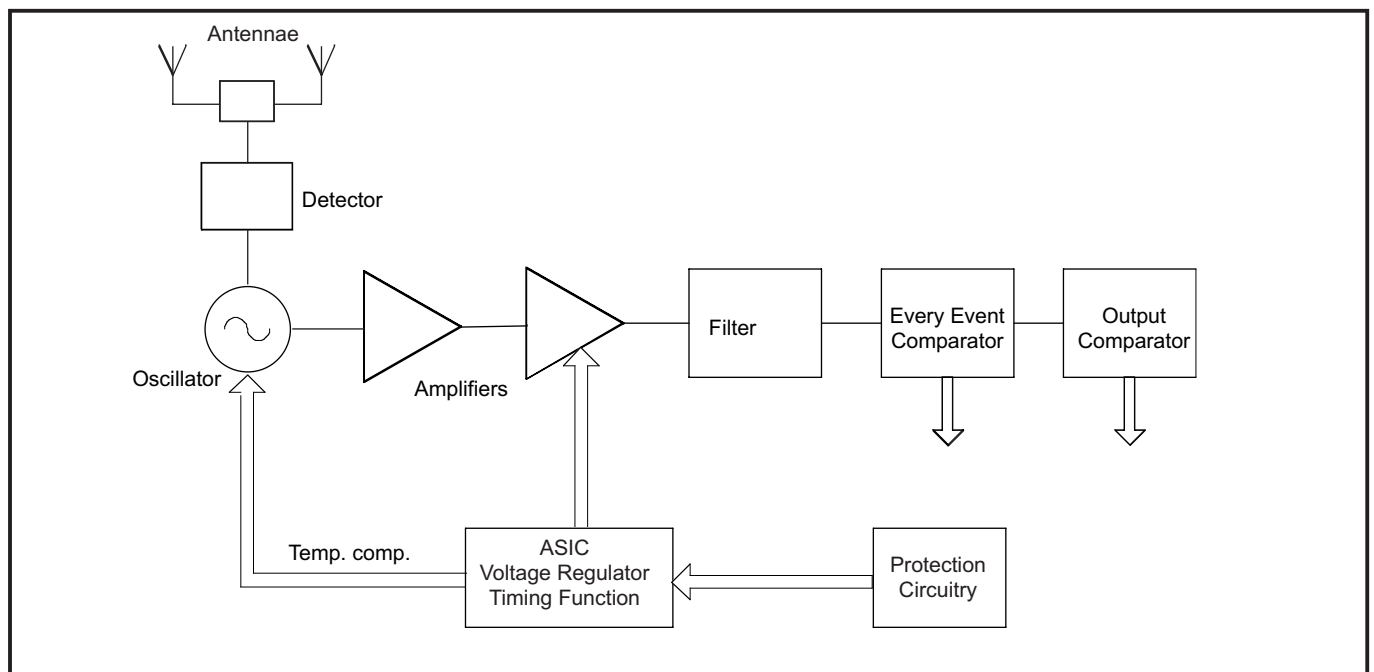
Fig. 1: MMS schematic
