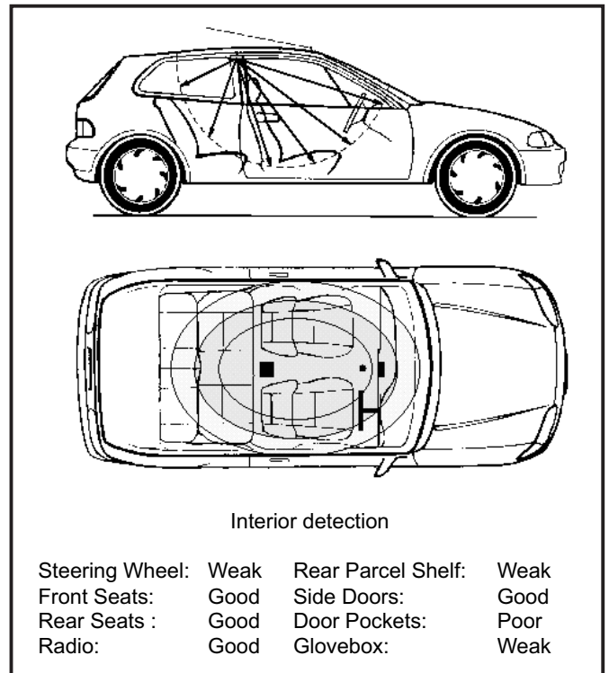
Fig. 2: Centre roof mounted
