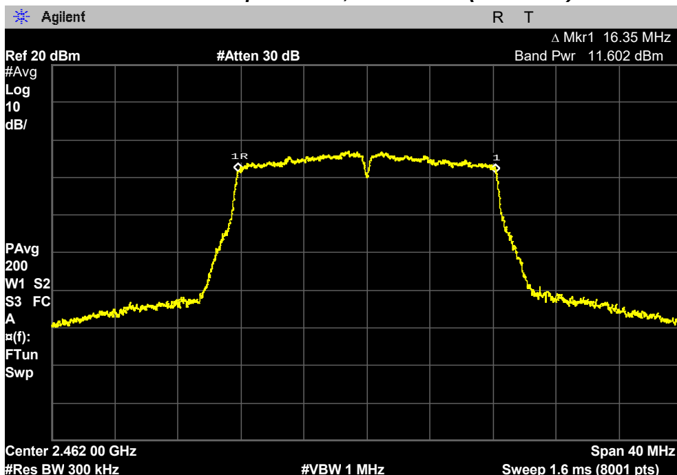
Maximum Conducted Output Power, 11 Channel (2462 MHz)
