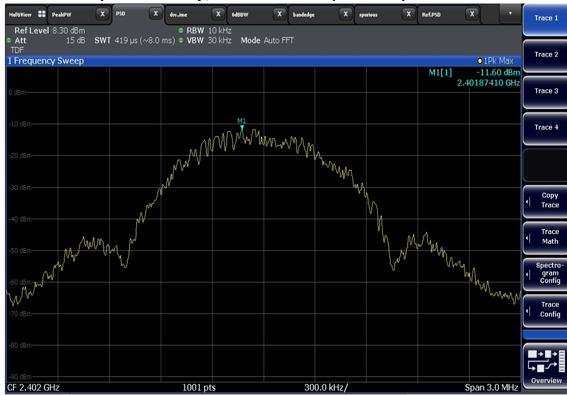
Peak Power Spectral Density, Lowest Channel (2402 MHz)
