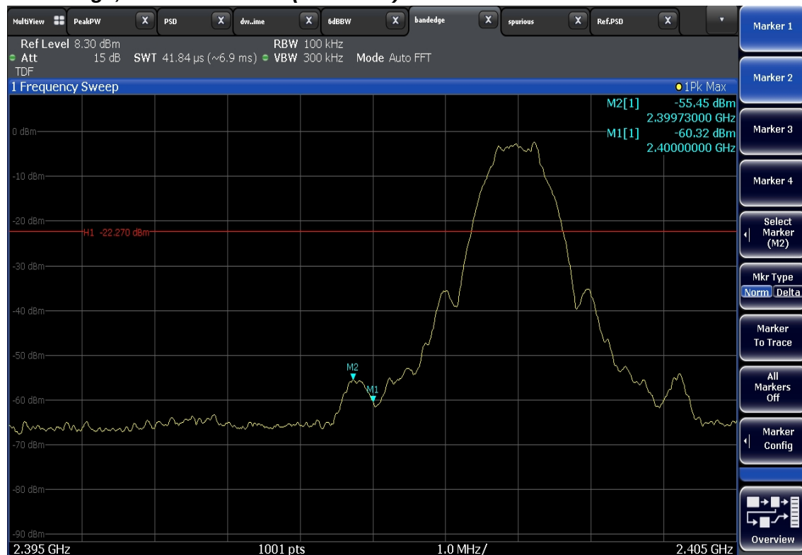
Band Edge, Lowest Channel (2402 MHz)
