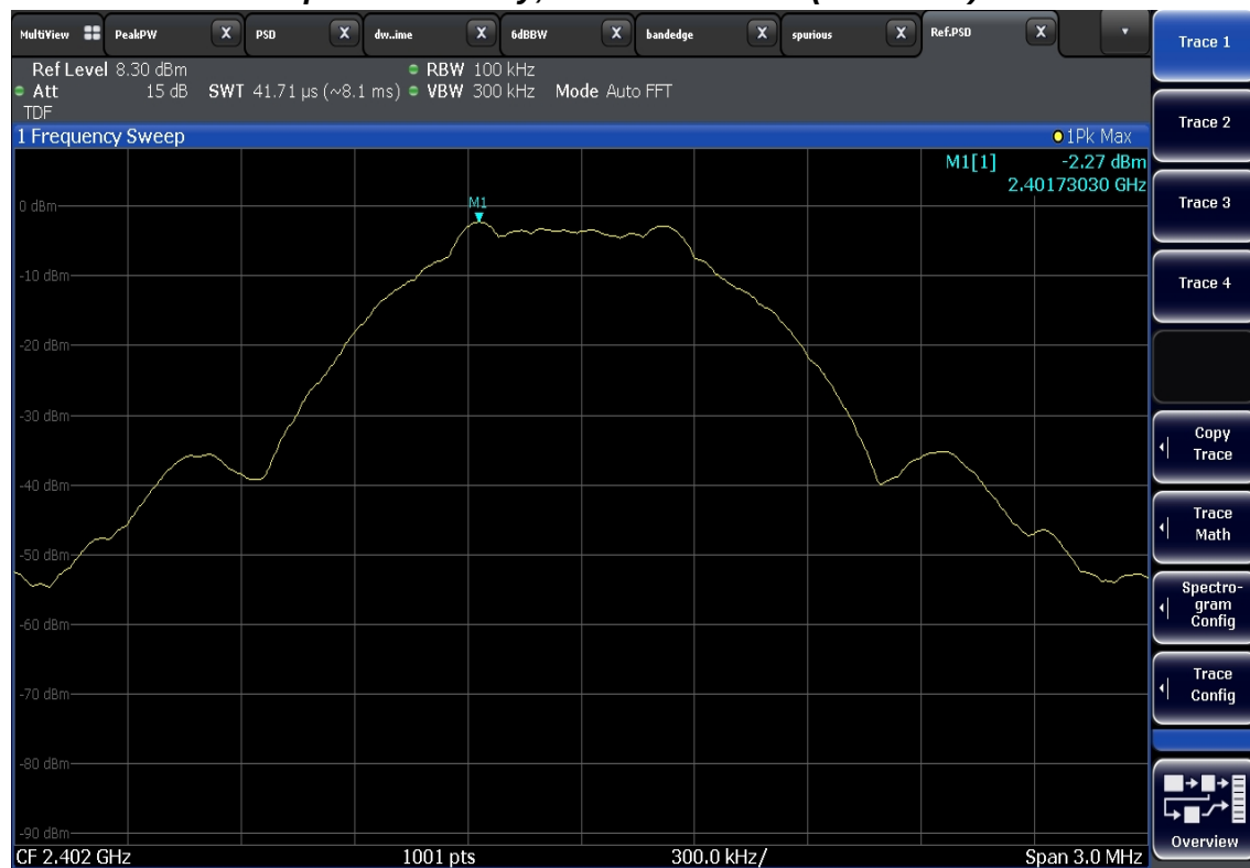
Reference Power Spectral Density, Lowest Channel (2402 MHz)
