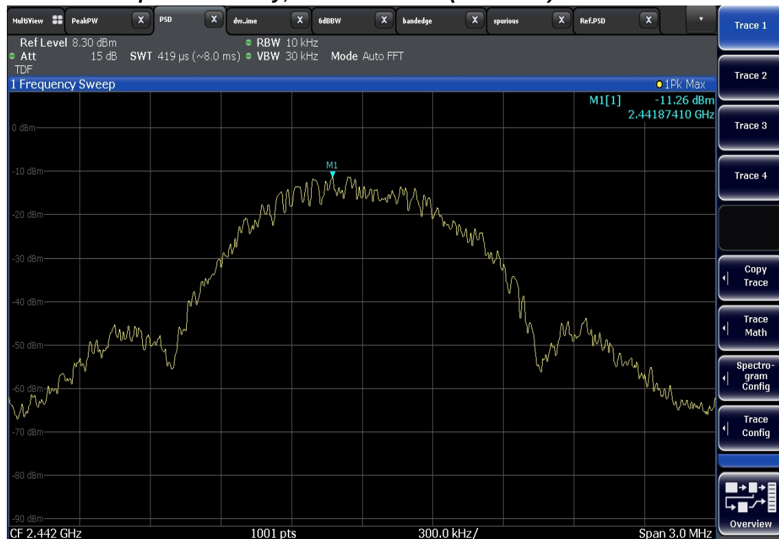
Peak Power Spectral Density, Middle Channel (2442 MHz)
