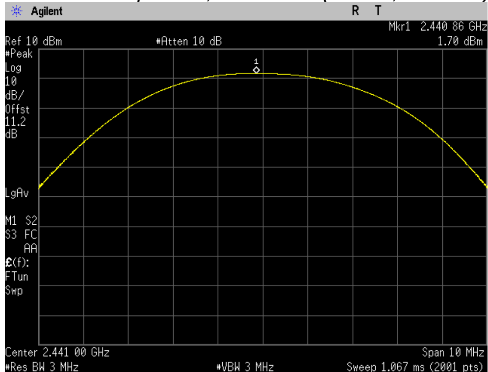
Maximum Peak Output Power, Middle channel (2441 MHz, GFSK mode)
