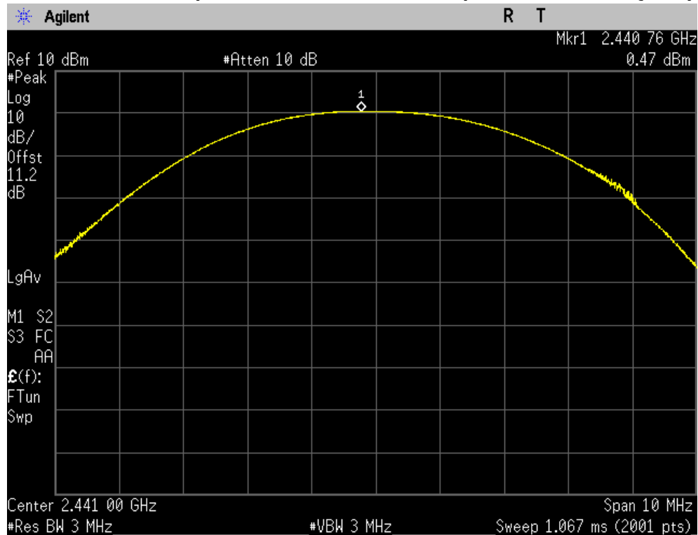
Maximum Peak Output Power, Middle channel (2441 MHz, \pi/4 DQPSK)
