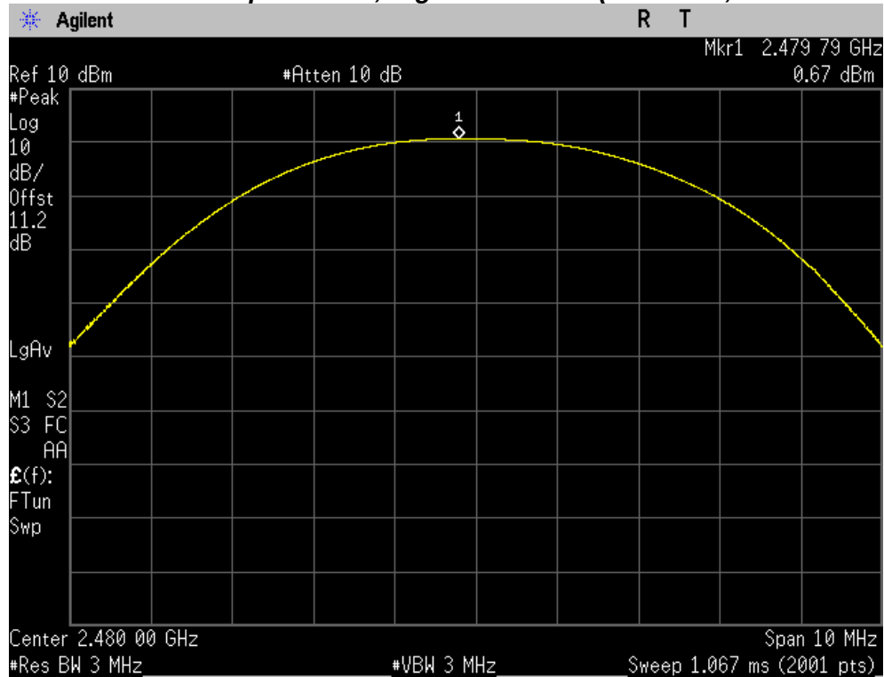
Maximum Peak Output Power, Highest channel (2480 MHz, GFSK mode)
