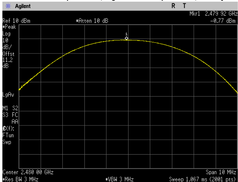
Maximum Peak Output Power, Highest channel (2480 MHz, \pi/4 DQPSK)
