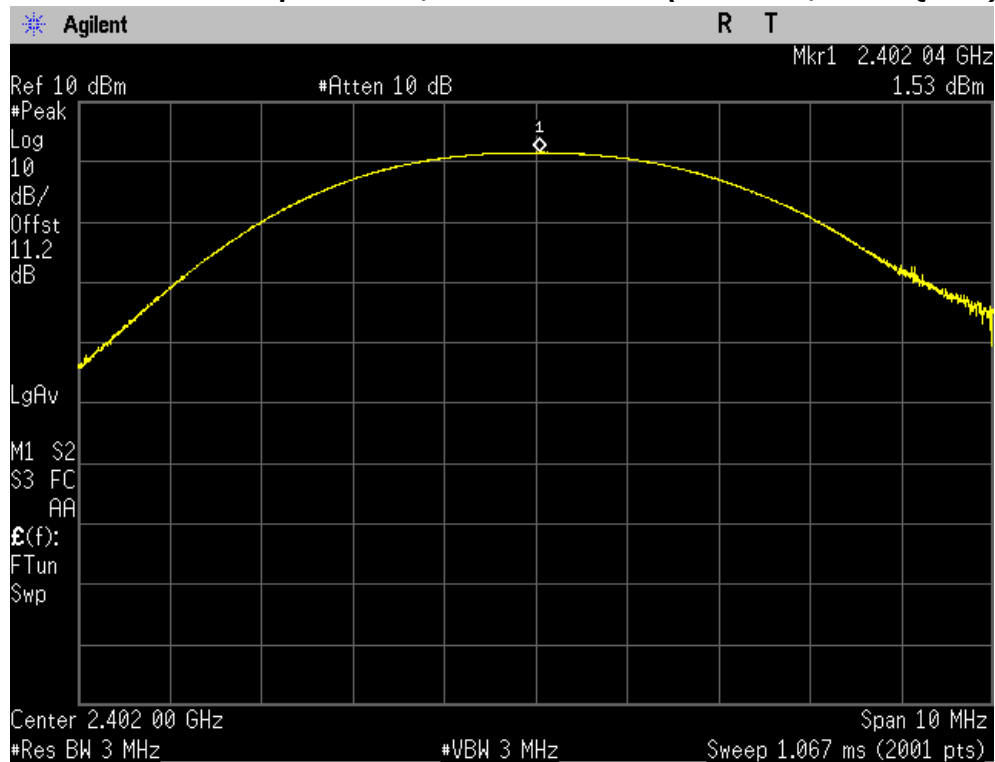
Maximum Peak Output Power, Lowest channel (2402 MHz, \pi/4 DQPSK)
