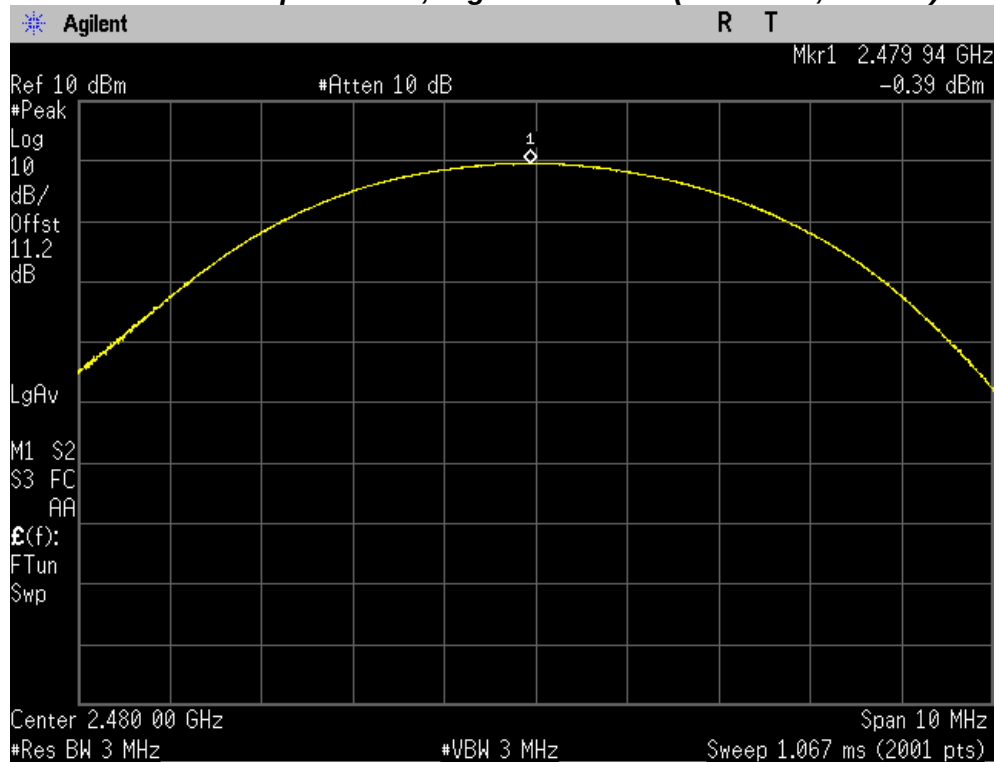
Maximum Peak Output Power, Highest channel (2480 MHz, 8DPSK)
