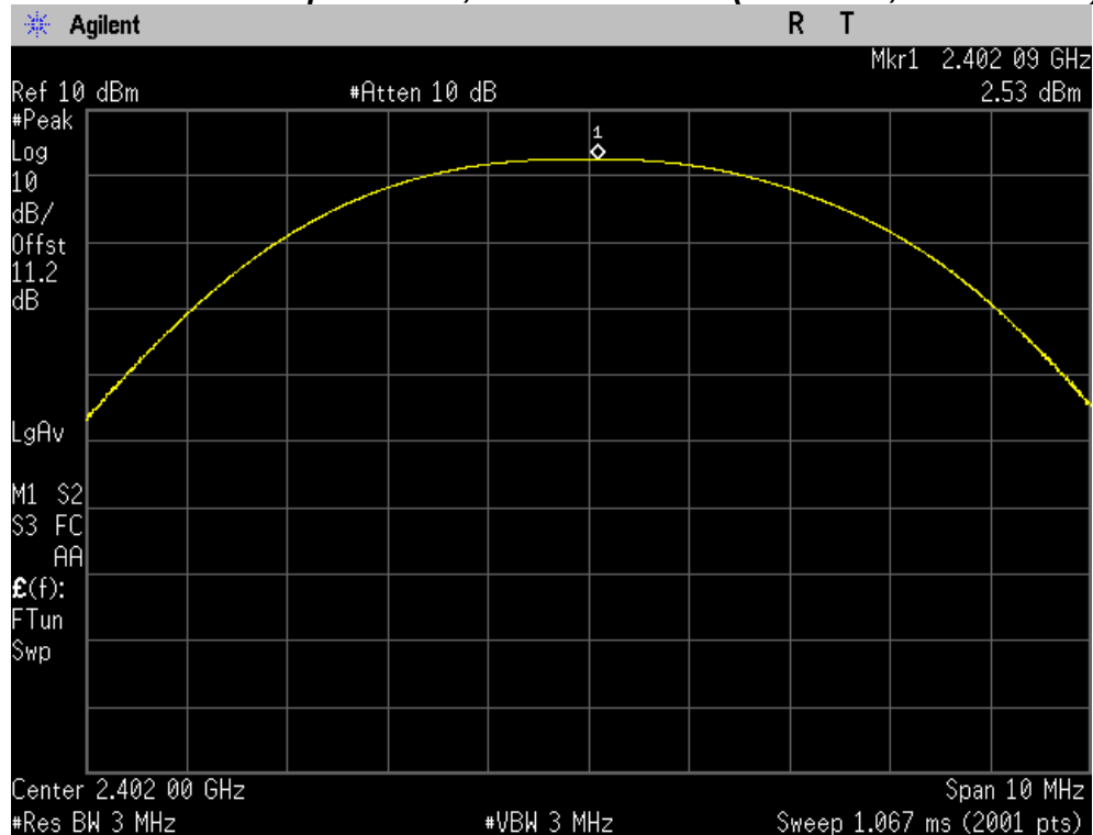
Maximum Peak Output Power, Lowest channel (2402 MHz, GFSK mode)
