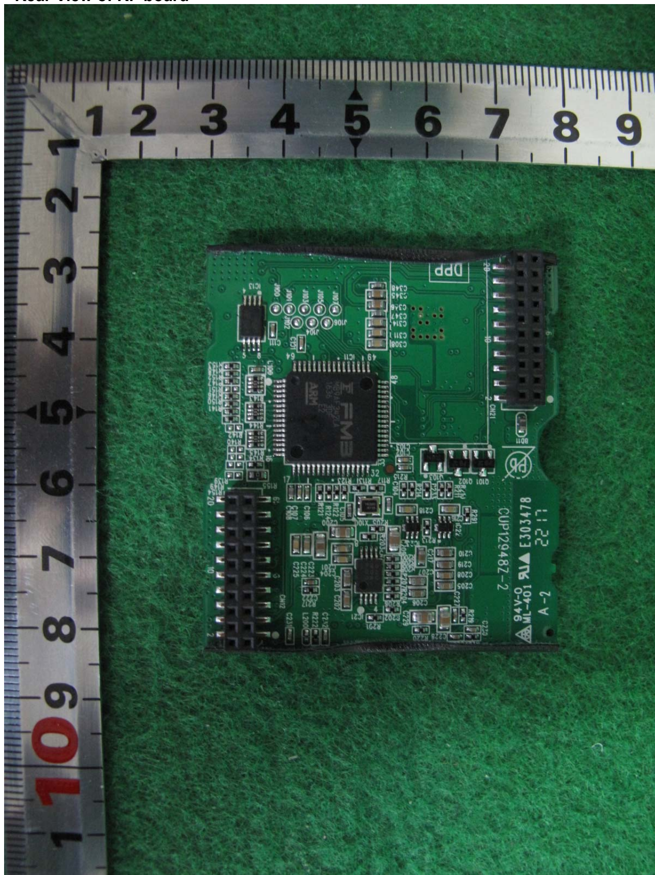
Rear View of RF board
