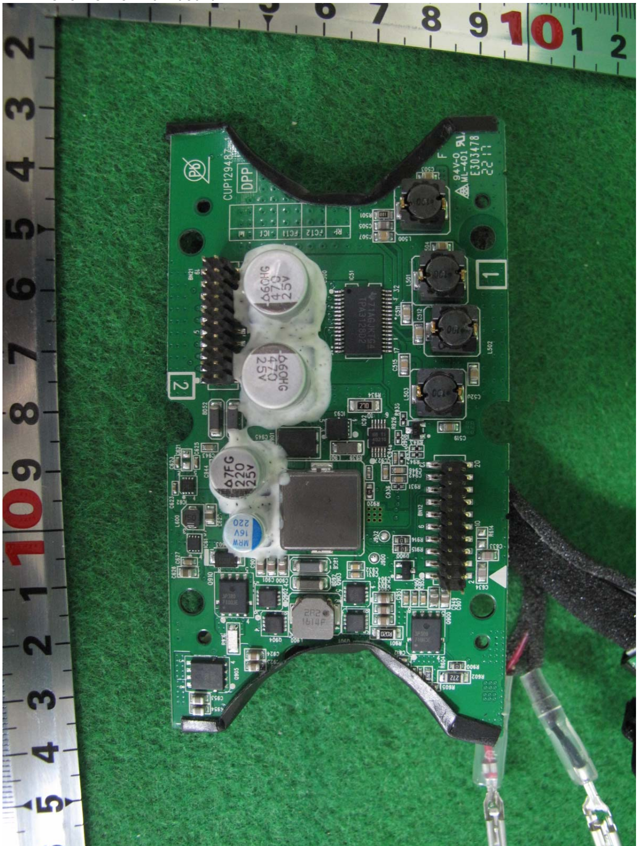
Front View of Mainboard
