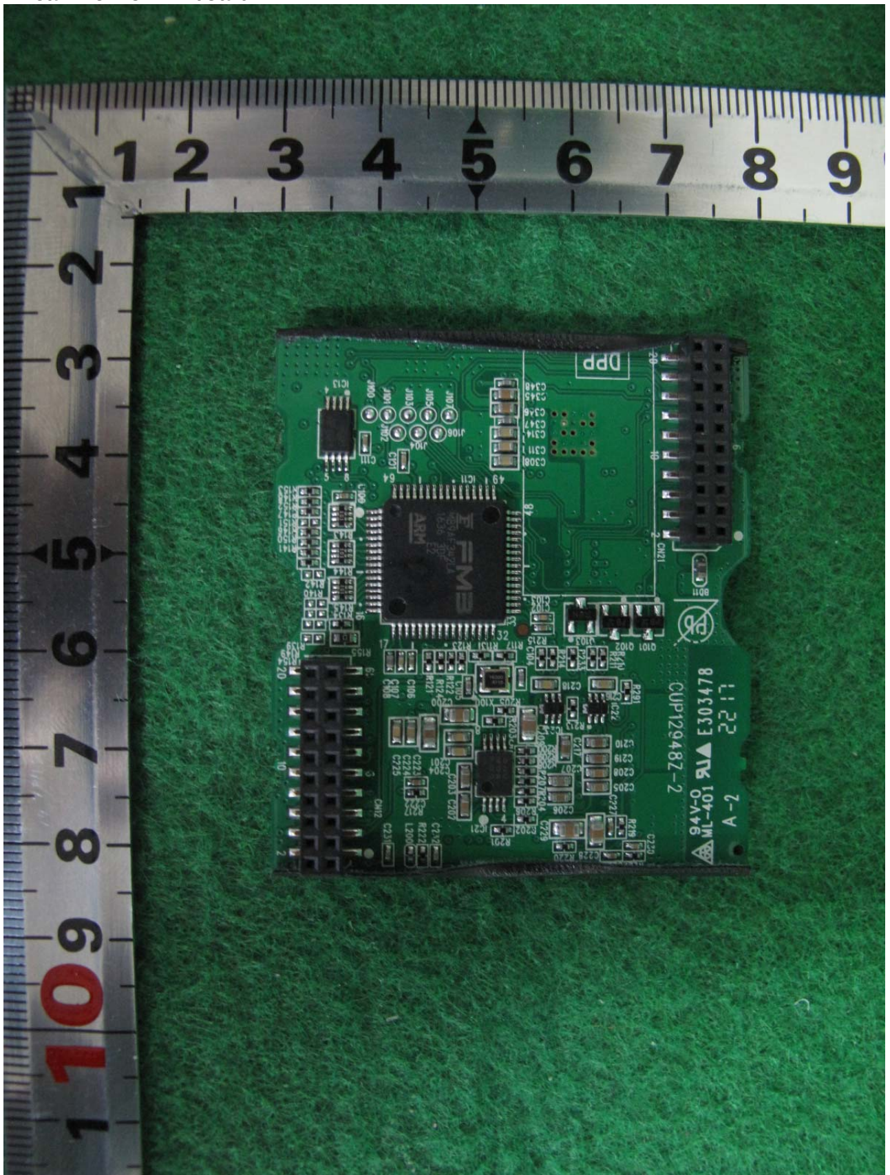
Rear View of RF board
