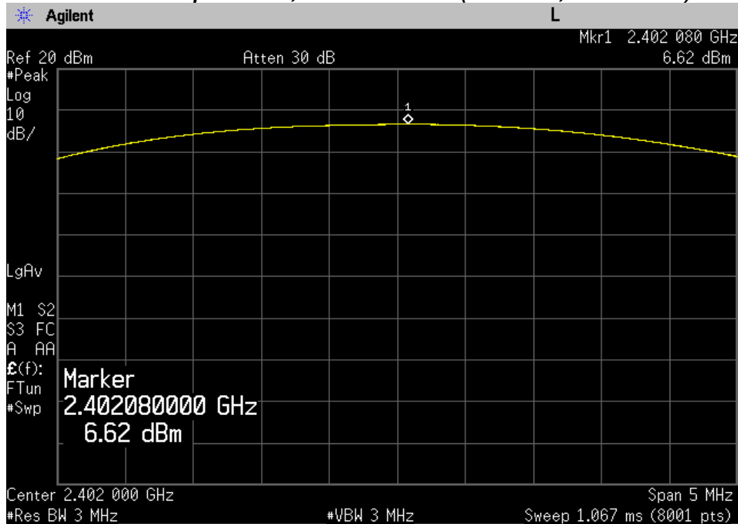
Maximum Peak Output Power, Lowest channel (2402 MHz, GFSK Mode)
