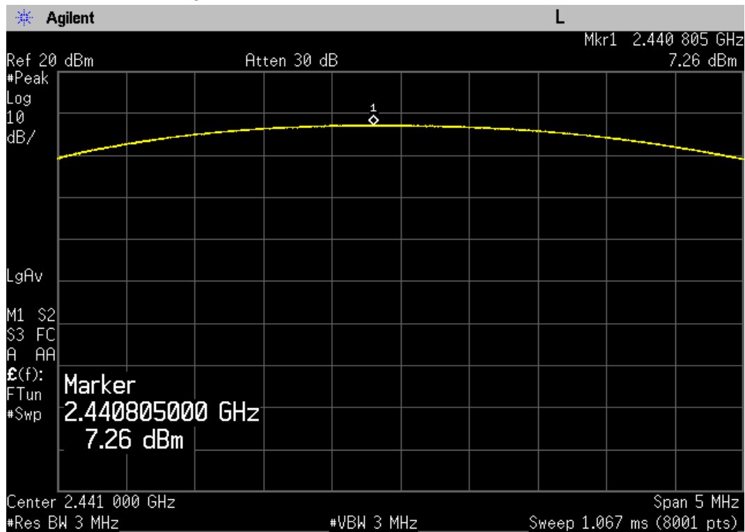
Maximum Peak Output Power, Middle channel (2441 MHz, \pi/4 DQPSK Mode)
