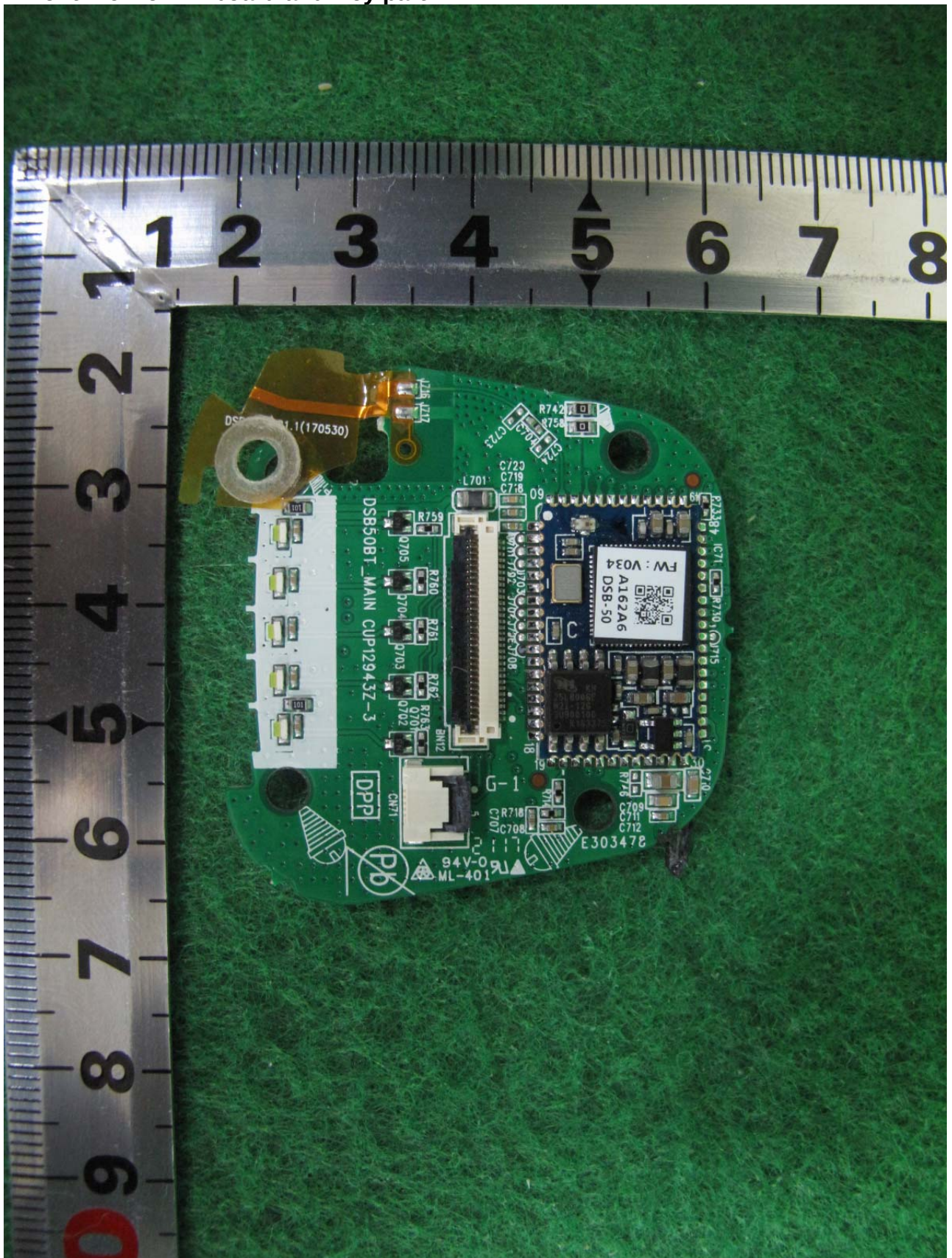
Front View of RF board and Key part
