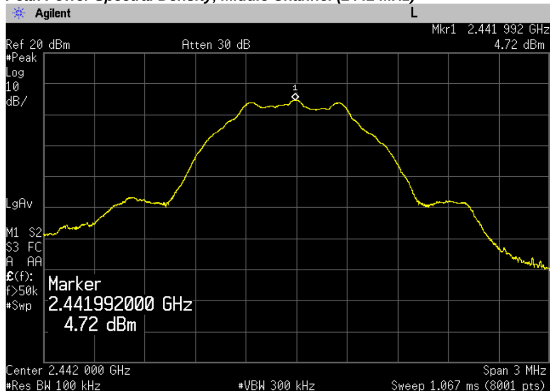
Peak Power Spectral Density, Middle Channel (2442 MHz)
