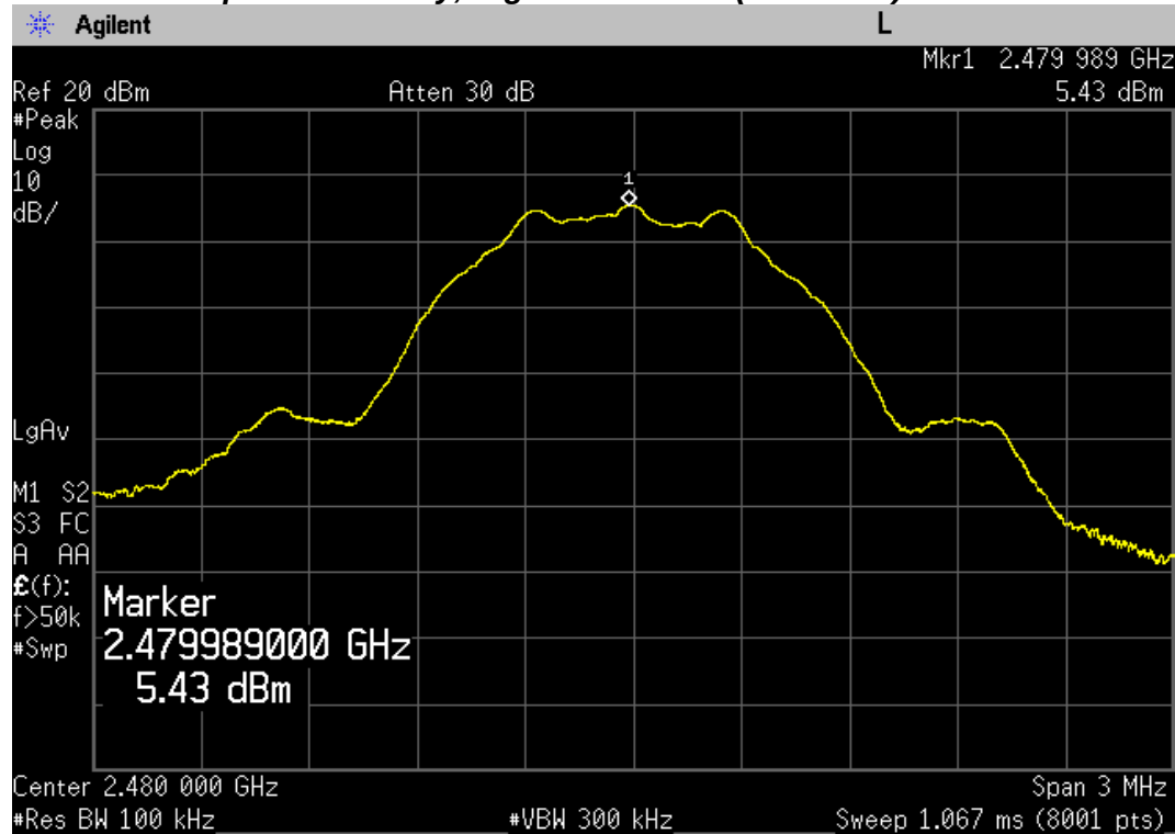
Peak Power Spectral Density, Highest Channel (2480 MHz)
