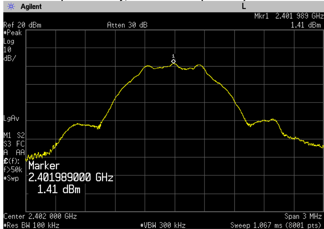
Peak Power Spectral Density, Lowest Channel (2402 MHz)
