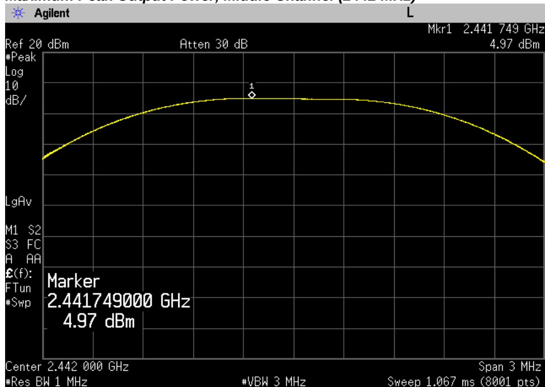
Maximum Peak Output Power, Middle Channel (2442 MHz)
