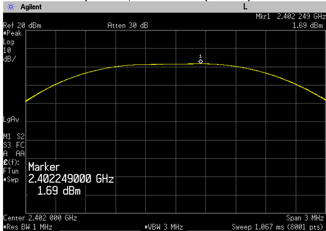
Maximum Peak Output Power, Lowest Channel (2402 MHz)
