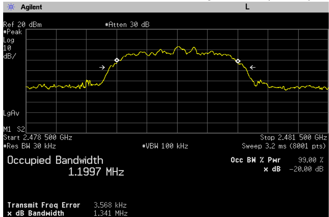
20 dB & 99% Bandwidth, \pi/4 DQPSK modulation, Highest Channel (2480 MHz)
