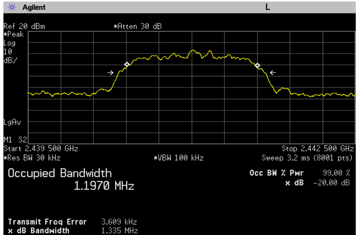
20 dB & 99% Bandwidth, \pi/4 DQPSK modulation, Middle Channel (2441 MHz)
