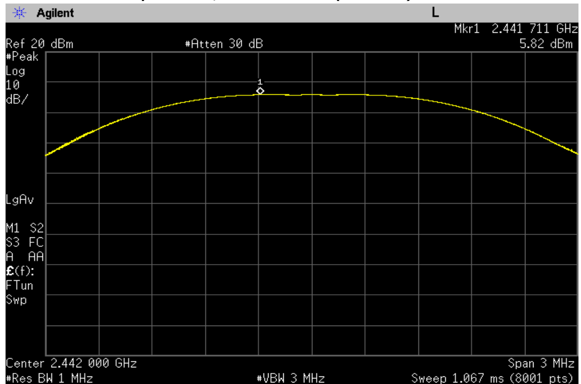
Maximum Peak Output Power, Middle Channel (2442 MHz)
