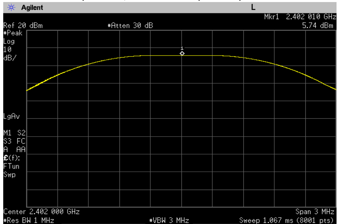
Maximum Peak Output Power, Lowest Channel (2402 MHz)
