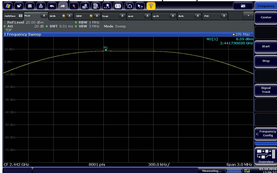
Maximum Peak Output Power, Middle Channel (2442 MHz)
